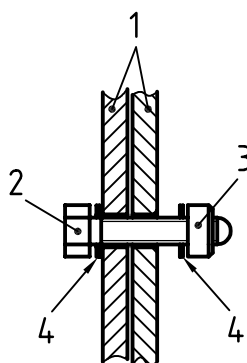
b) Bolt connection detail
