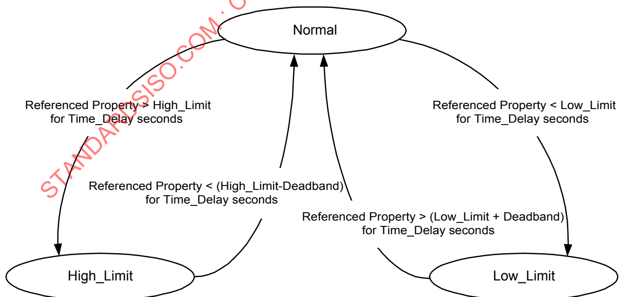
Figure 13-8. OUT_OF_RANGE algorithm.
