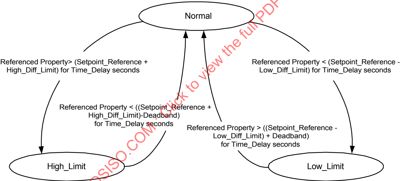
Figure 13-6. FLOATING_LIMIT algorithm.
