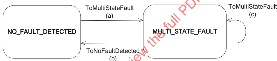
Figure 13-25. Transitions indicated by FAULT_CHARACTERSTRING algorithm
