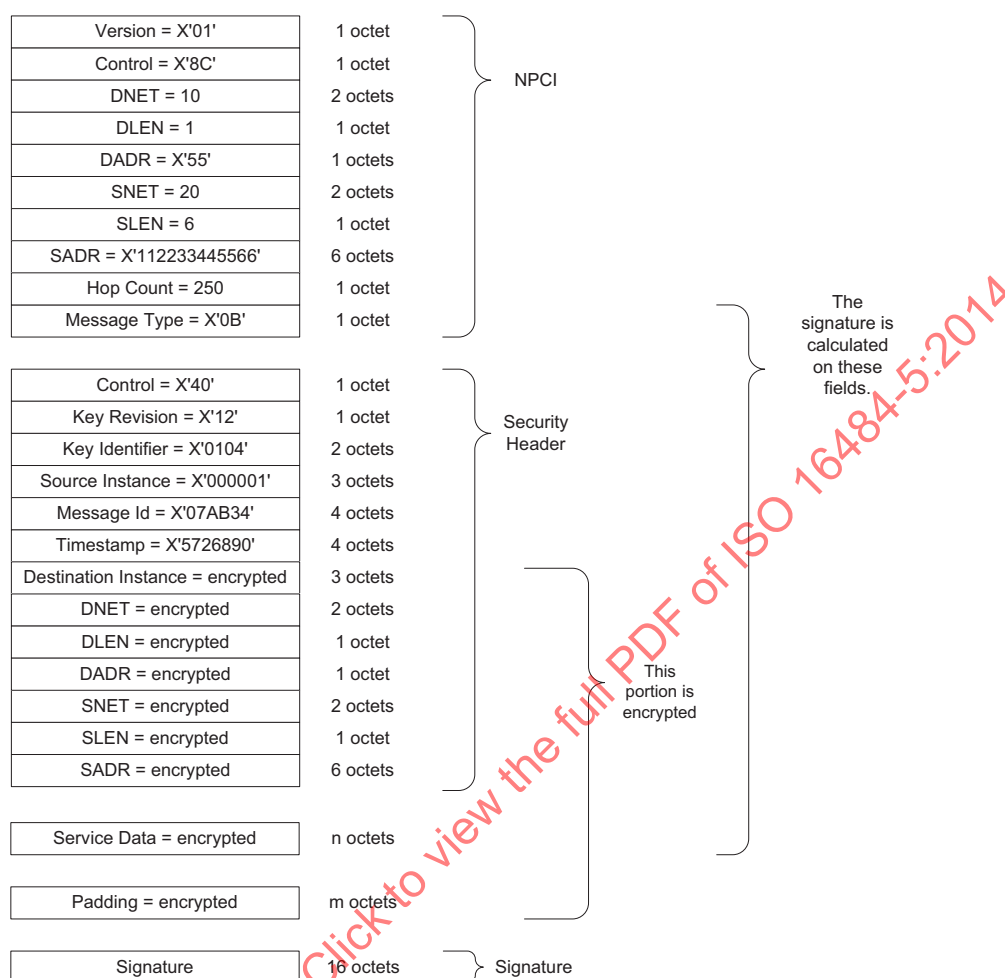
Figure 24-5. An example encrypted message.
