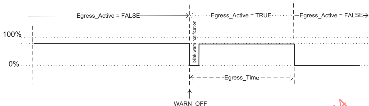
Figure 12-15. Blink-warn and Egress Time
