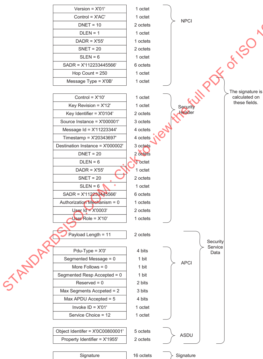
Figure 24-1. An example secured APDU (Read-Property).
