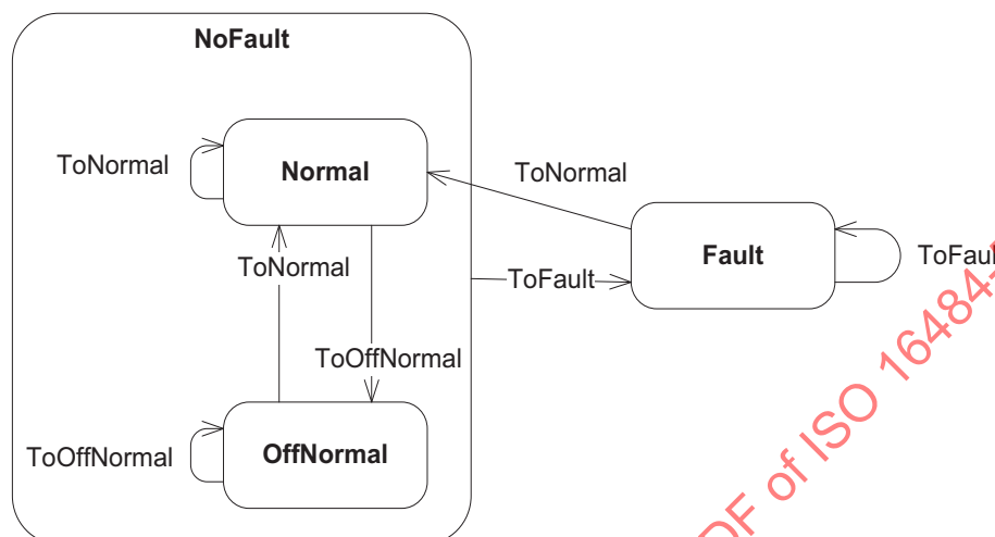
Figure 13-3. Event-State-Detection State Machine
