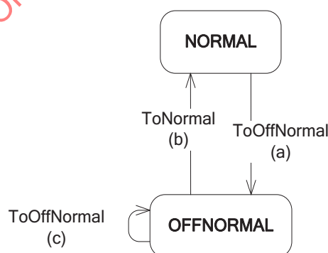
Figure 13-8. Transitions indicated by CHANGE_OF_BITSTRING algorithm
