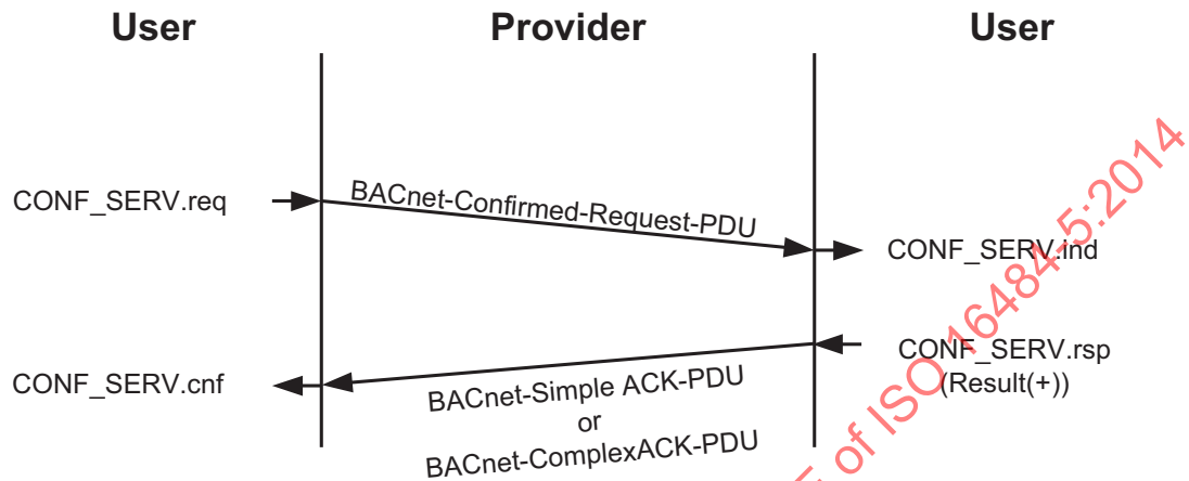
Figure 5-6. Time sequence diagram for normal confirmed services.
