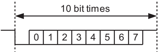
Figure 9-2. Octet framing.
