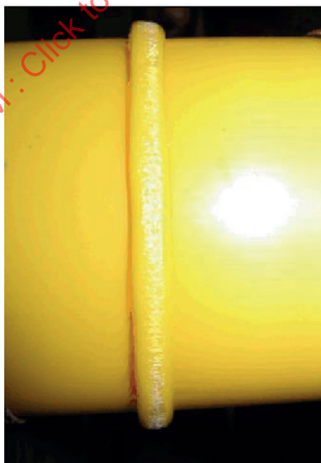
Figure 4 — Typical single bead shape around the entire pipe circumference
