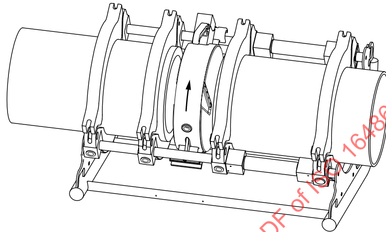
Figure A.3 — Planing the pipe or spigot ends by the planing tool between the ends
