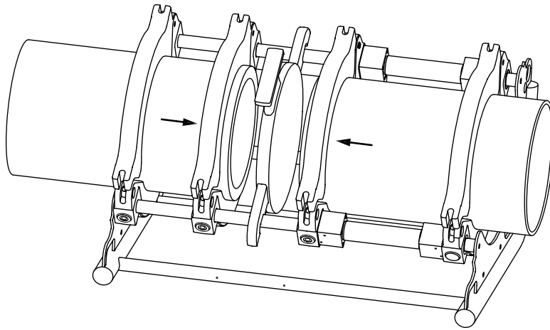
Figure A.4 — Heating the spigot ends
