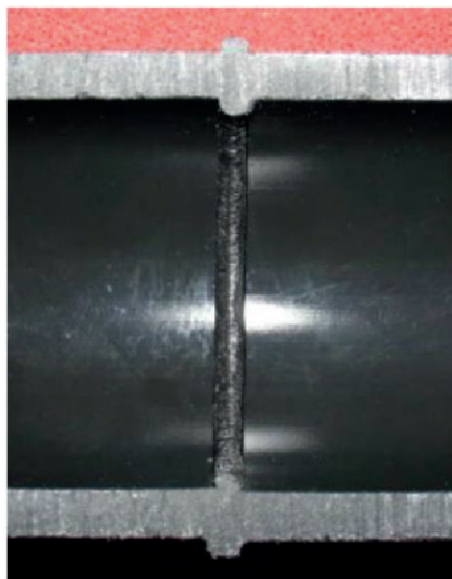
Figure 5 — Typical single bead shape in a sectioned joint
