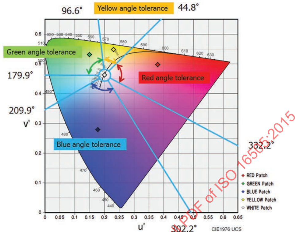
Figure 21 — Tolerance of colour deviation on the CIE 1976 UCS chromaticity diagram
