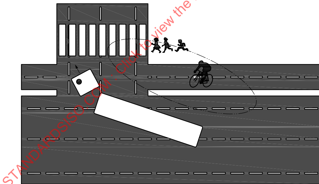
Figure B.29 — Turning left or right around corners with a connected trailer
