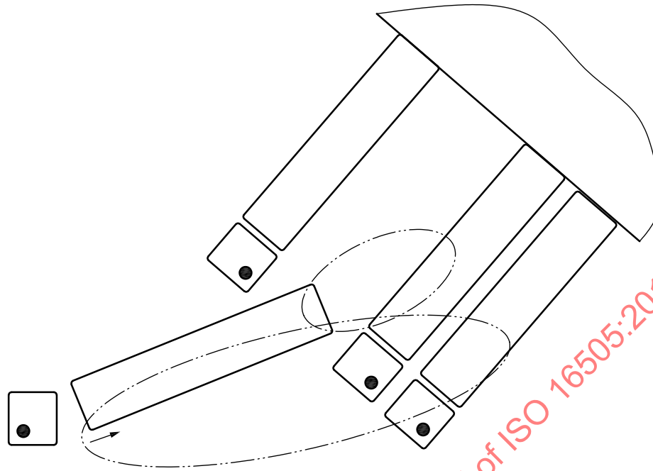
Figure B.28 — Manoeuvring towards an exact location for leaving or picking up people and/or goods
