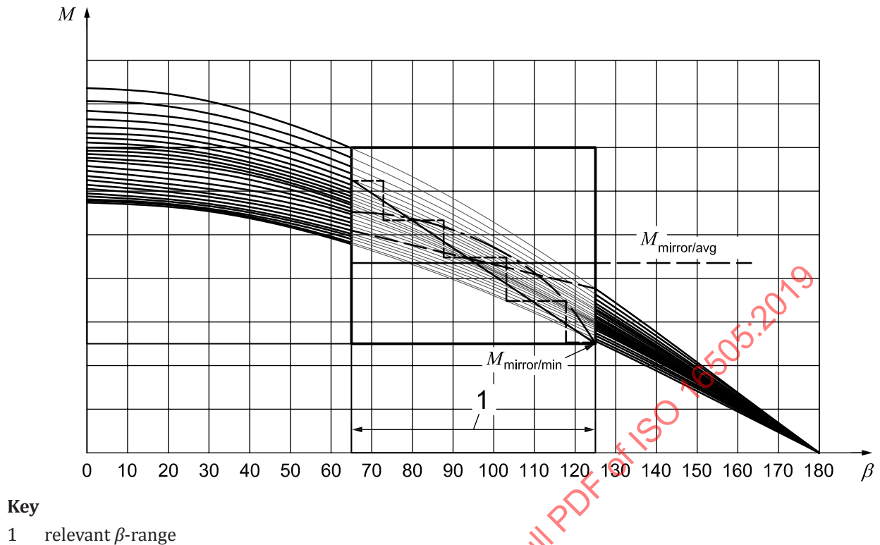
Figure B.22 — Examples of possible magnification factor variations
