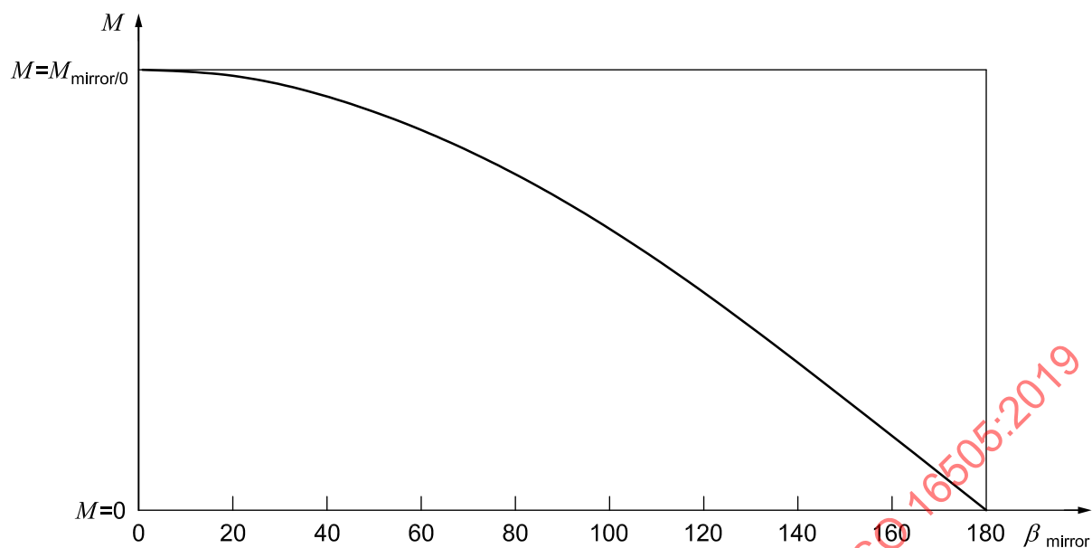
Figure B.16 — Magnification factor variation depending on total viewing angle, \beta (with d_{\text{object}} = \infty )
