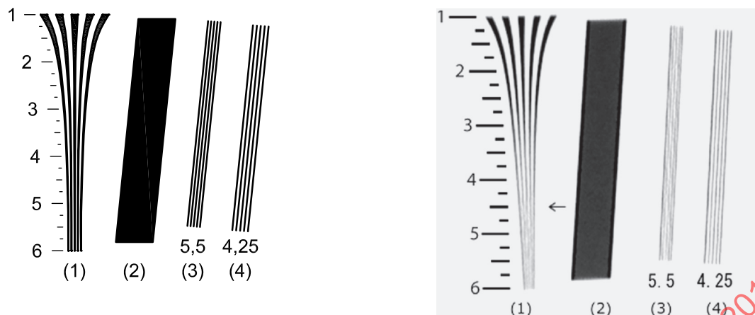
Figure 27 — Example of an original (left) and captured resolution chart (right)
