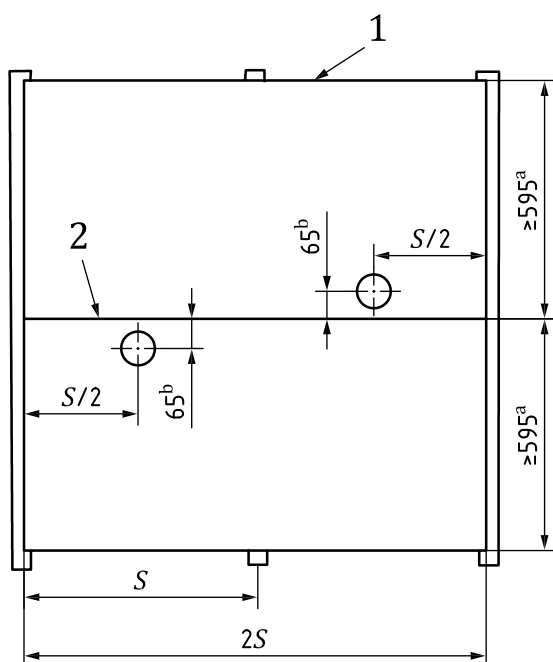
a) Edges partially supported
