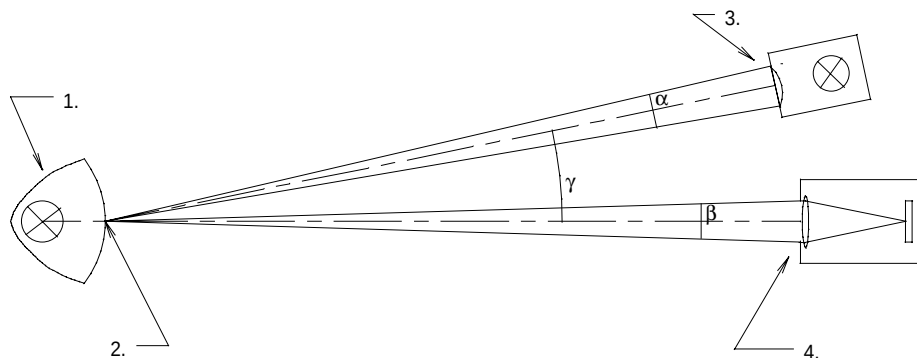
Figure A.1 - Schematic test set-up for determining phantom signal ratio.
