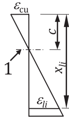
b) Strain distribution
