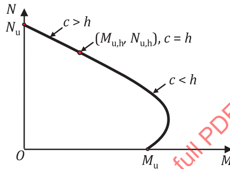
Figure 17 — N - M relationship
