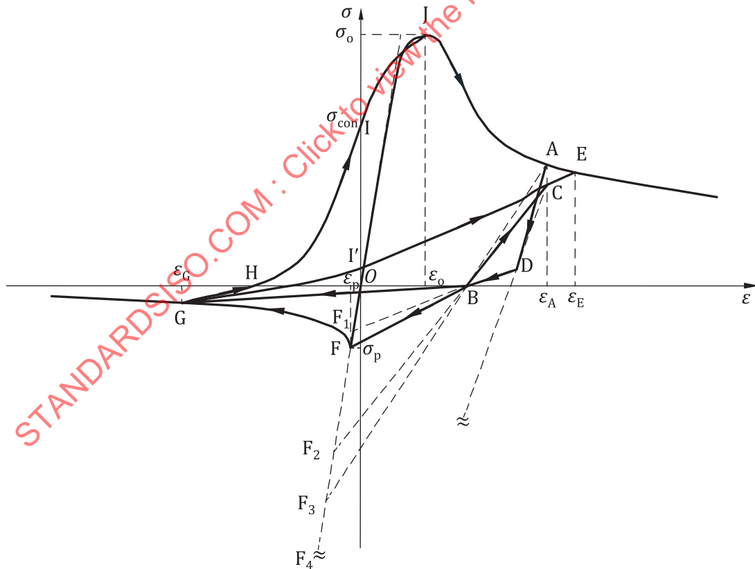
Figure 10 — Schematic diagram of stress-strain hysteretic relationship of concrete
