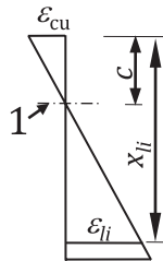
b) Strain distribution
