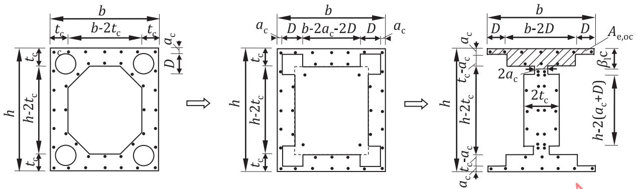
a) Simplification of cross-section
