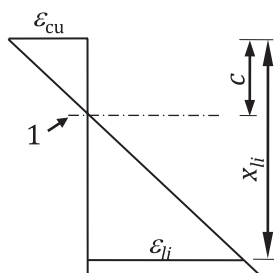
b) Strain distribution
