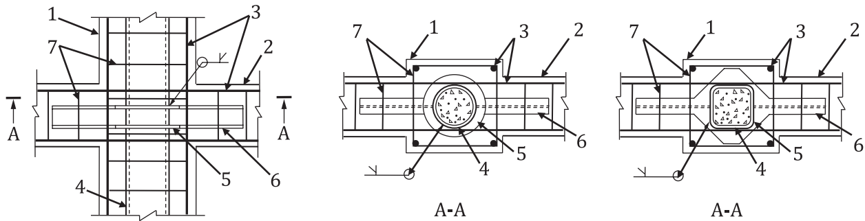
a) When the spacing between the longitudinal reinforcement of the beam is greater than the outside diameter (width/height) of the steel tube
