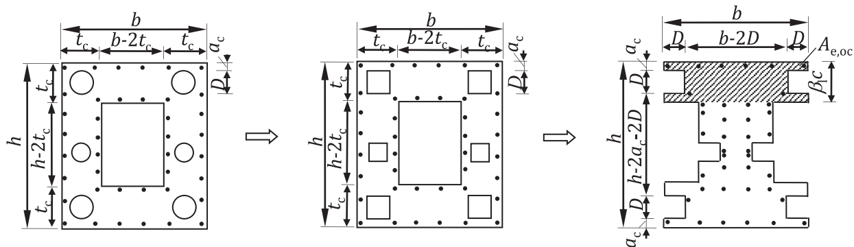
a) Simplification of cross-section
