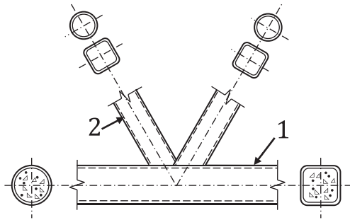
a) Overlap K-joint
