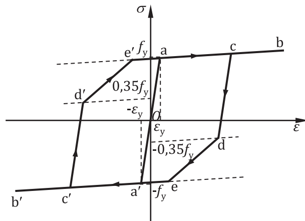
Figure 11 — Schematic diagram of stress-strain hysteretic relationship of structural steel
