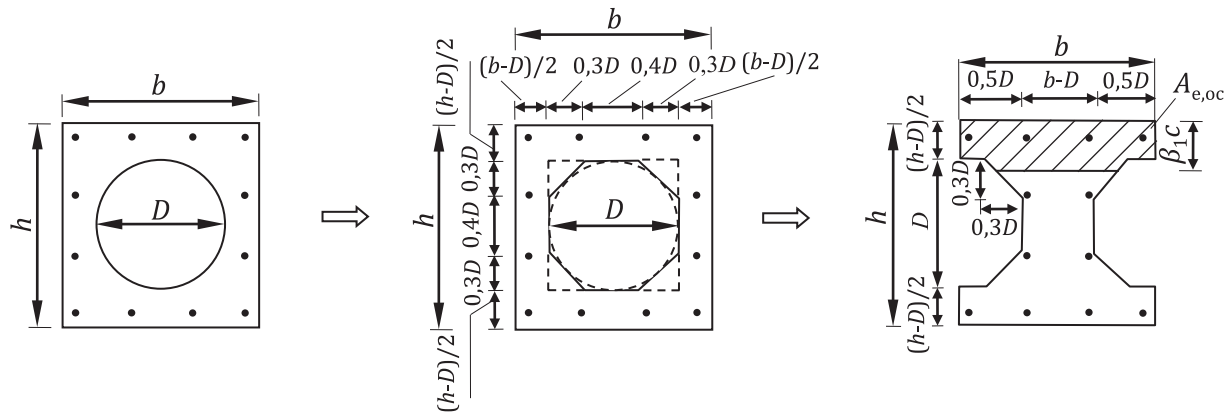
a) Simplification of cross-section
