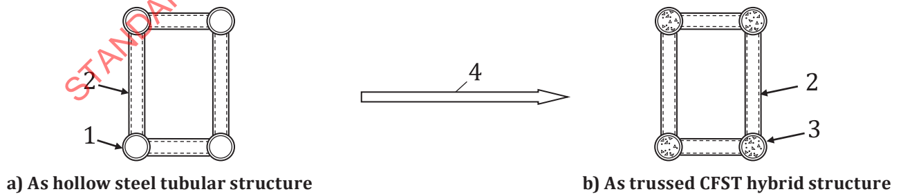
Figure 2 — Cross-sections of trussed CFST hybrid structures with square or rectangular CFST members
