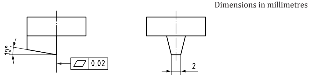
Figure 1 — Form of the striker
