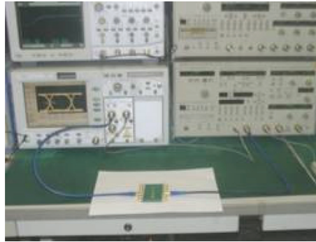
Figure 10 — Example of set-up for measurement of eye patterns
