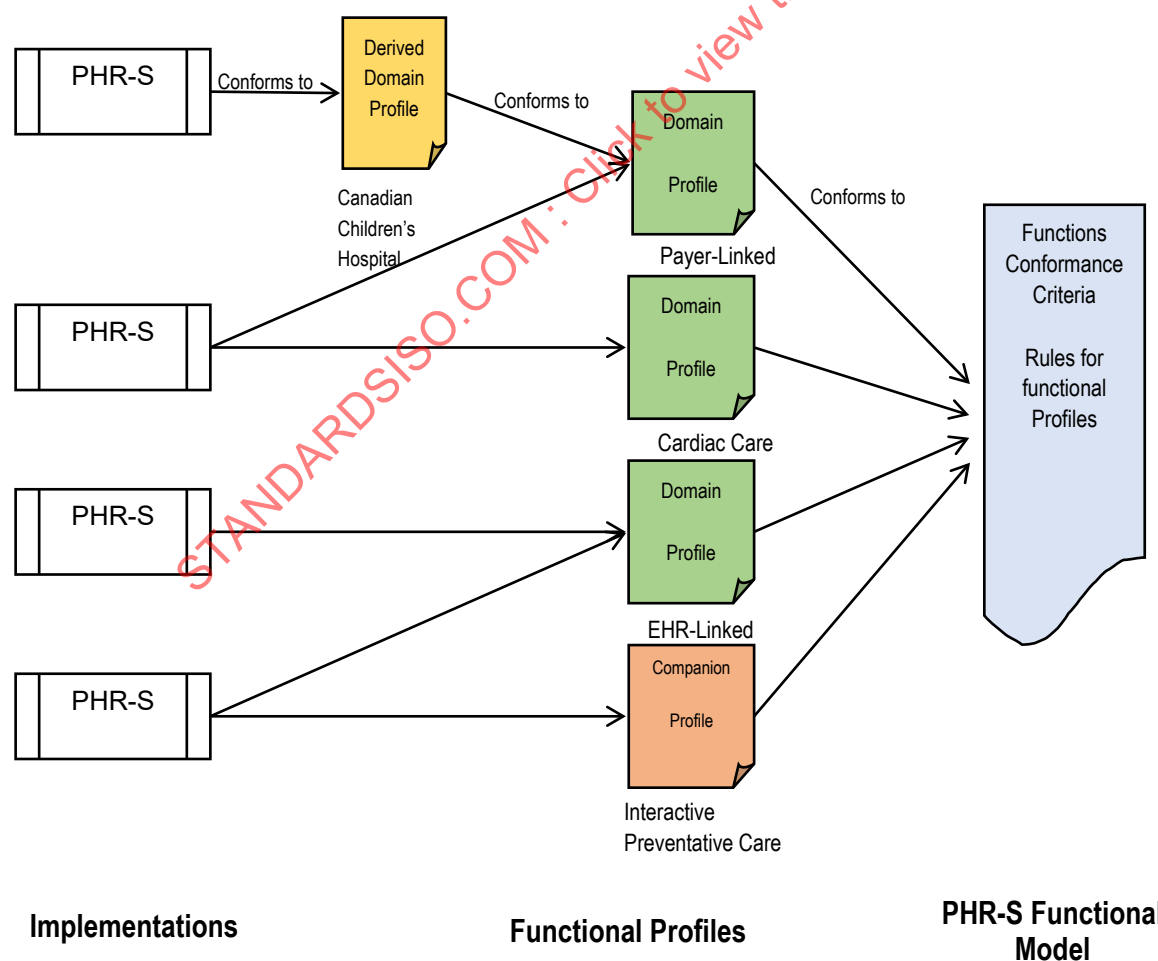
Figure 3: Conformance Relationships
