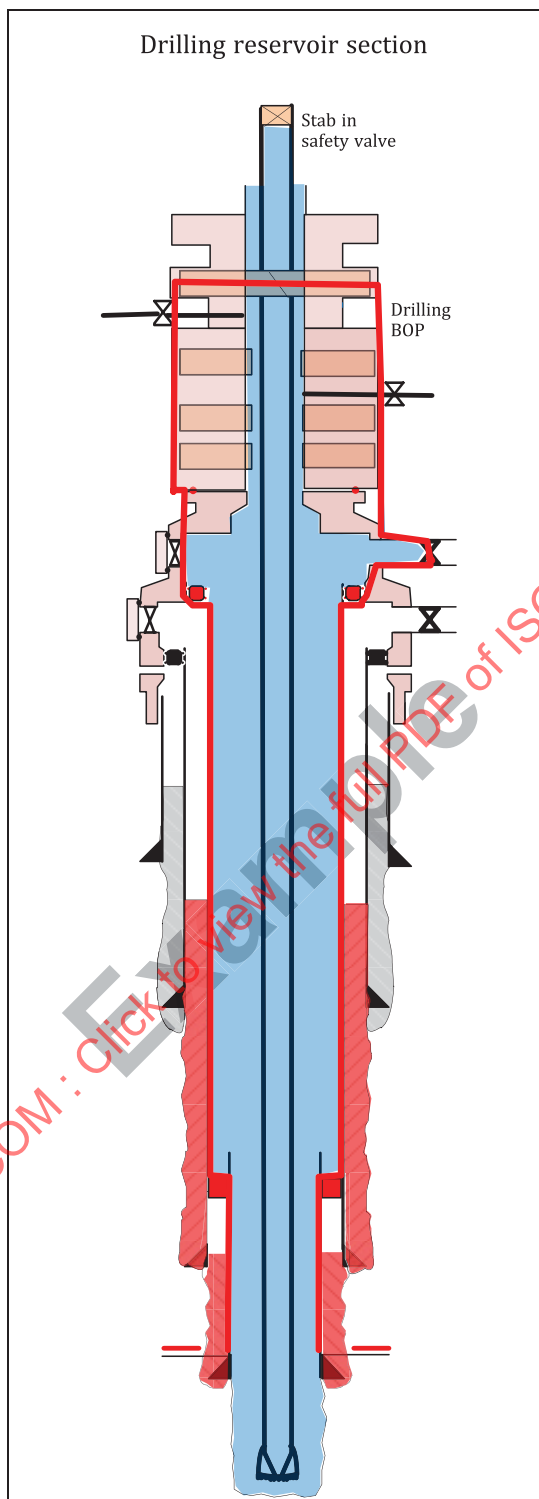
Figure F.2 — Example of well barriers during the construction phase
