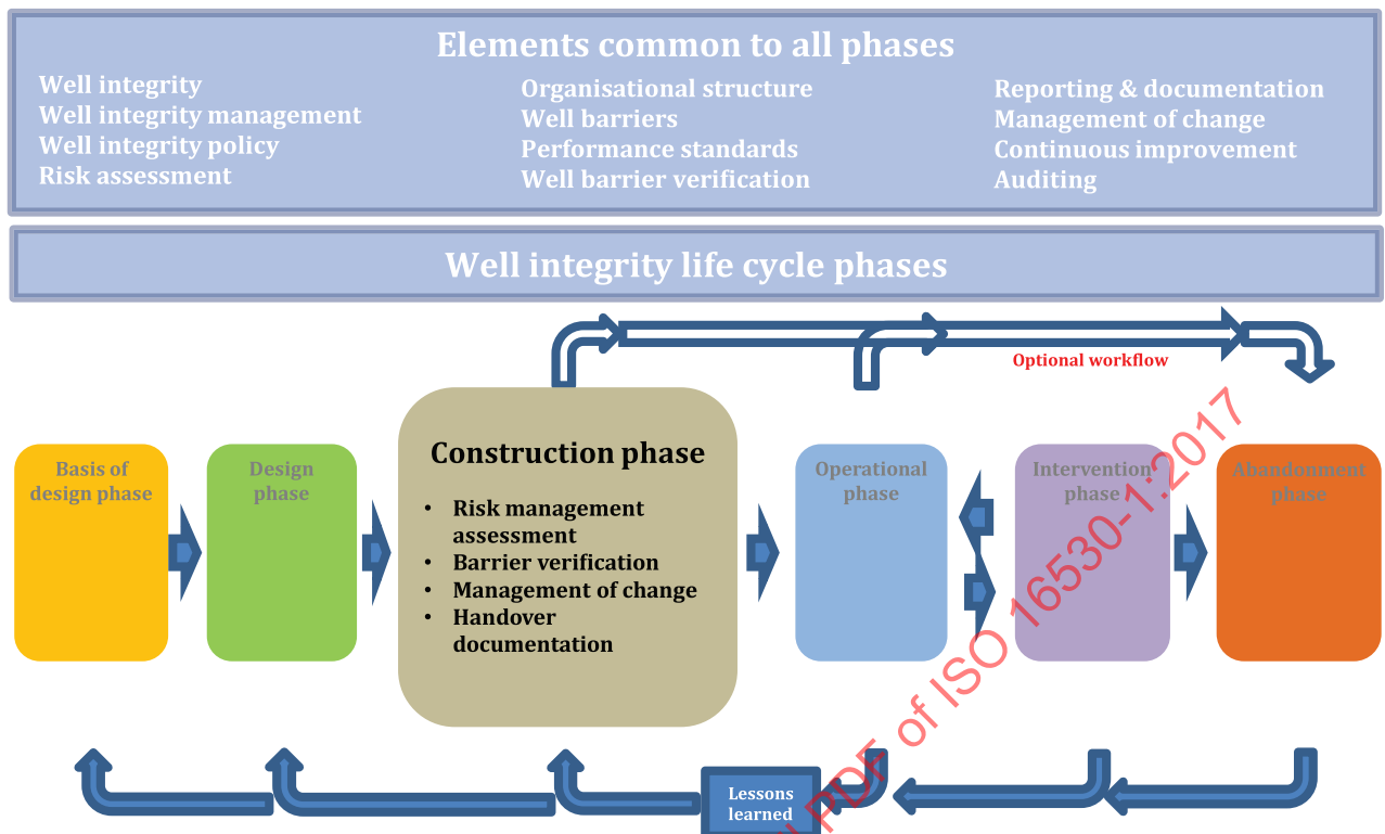
Figure 5 — Well construction phase
