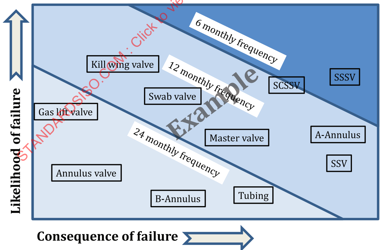
Figure 7 — Example of risk-based model as applied to well integrity assurance activities
