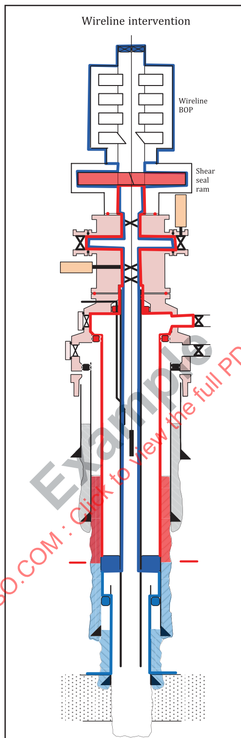
Figure F.3 — Example of well barriers during the intervention phase
