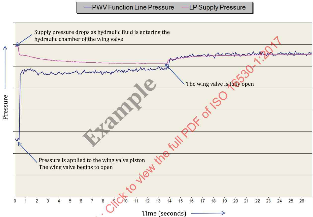
Figure H.2 — Signature of a production wing valve (PWV)
