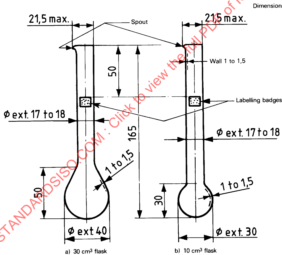
Figure 3 — Digestion flasks for the semi-micro method
