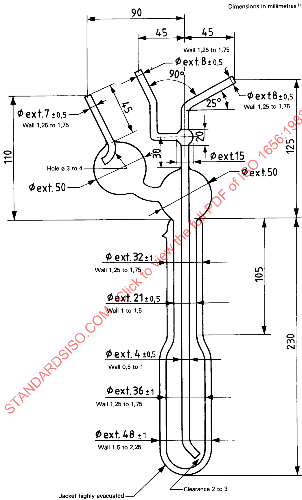
Figure 5 — Distillation flask for the semi-micro method
