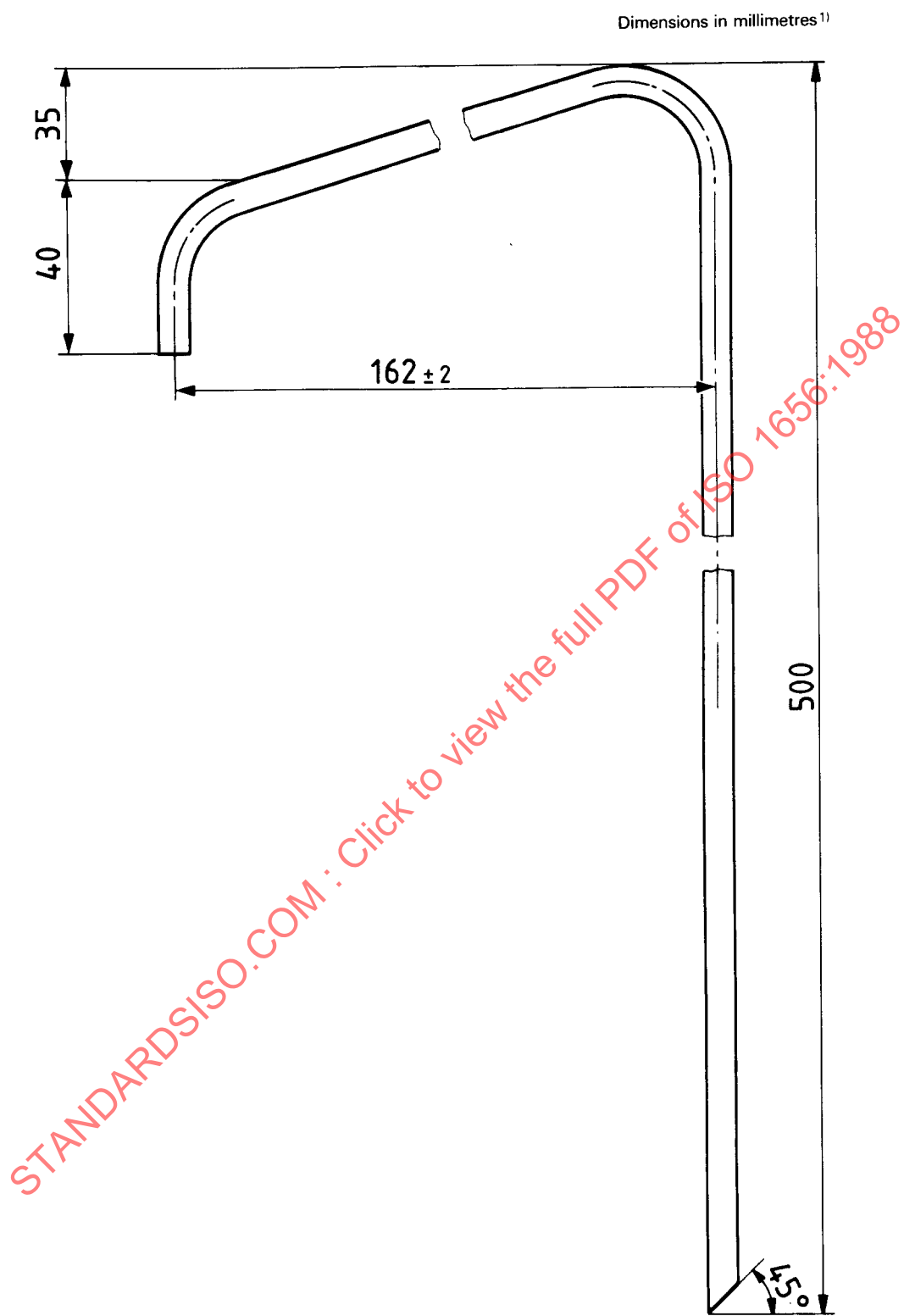
Figure 9 — Condenser tube for the semi-micro method
