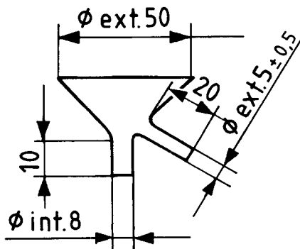
Figure 8 — Drip funnel for the semi-micro method
