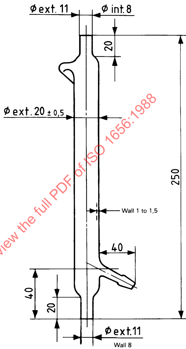
Figure 7 — Condenser jacket for the semi-micro method
