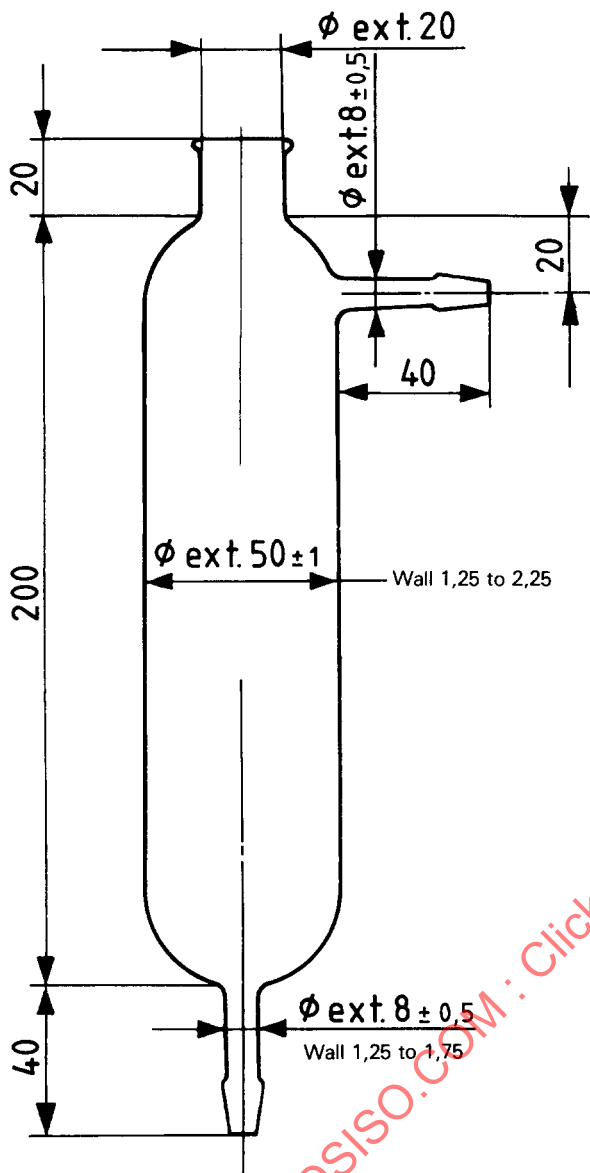
Figure 6 — Trap for the semi-micro method
