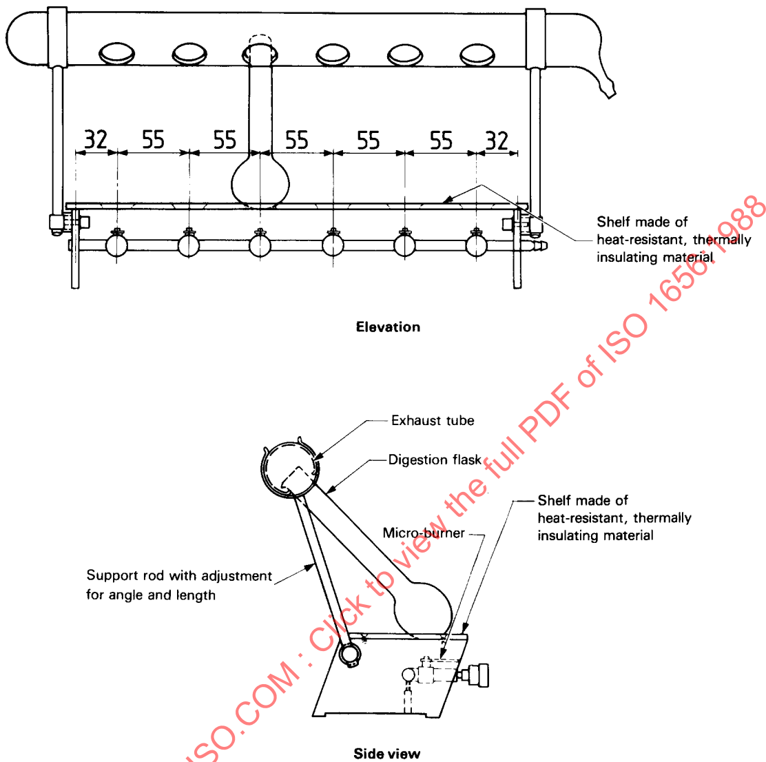
Figure 1 — Assembly of digestion apparatus for the semi-micro method
