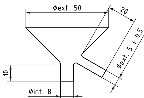
Figure 8 — Condenser jacket for the semi-micro method
