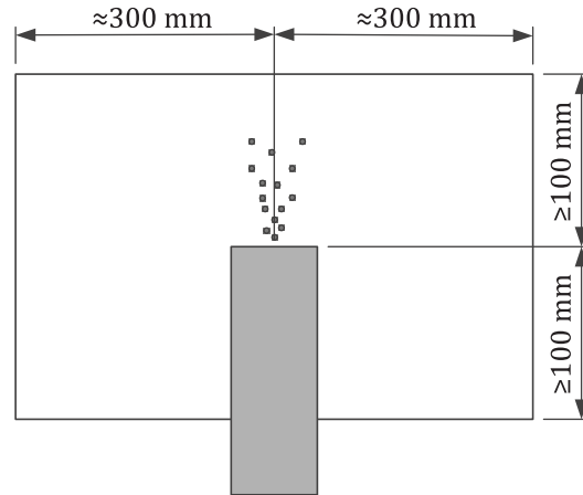
Figure C.3 — Aerosol outlet orifice positioning within the test chamber
