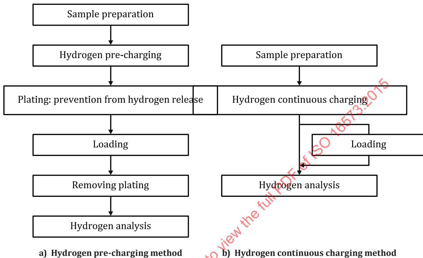
Figure 1 — Flow chart illustrating the test methods
