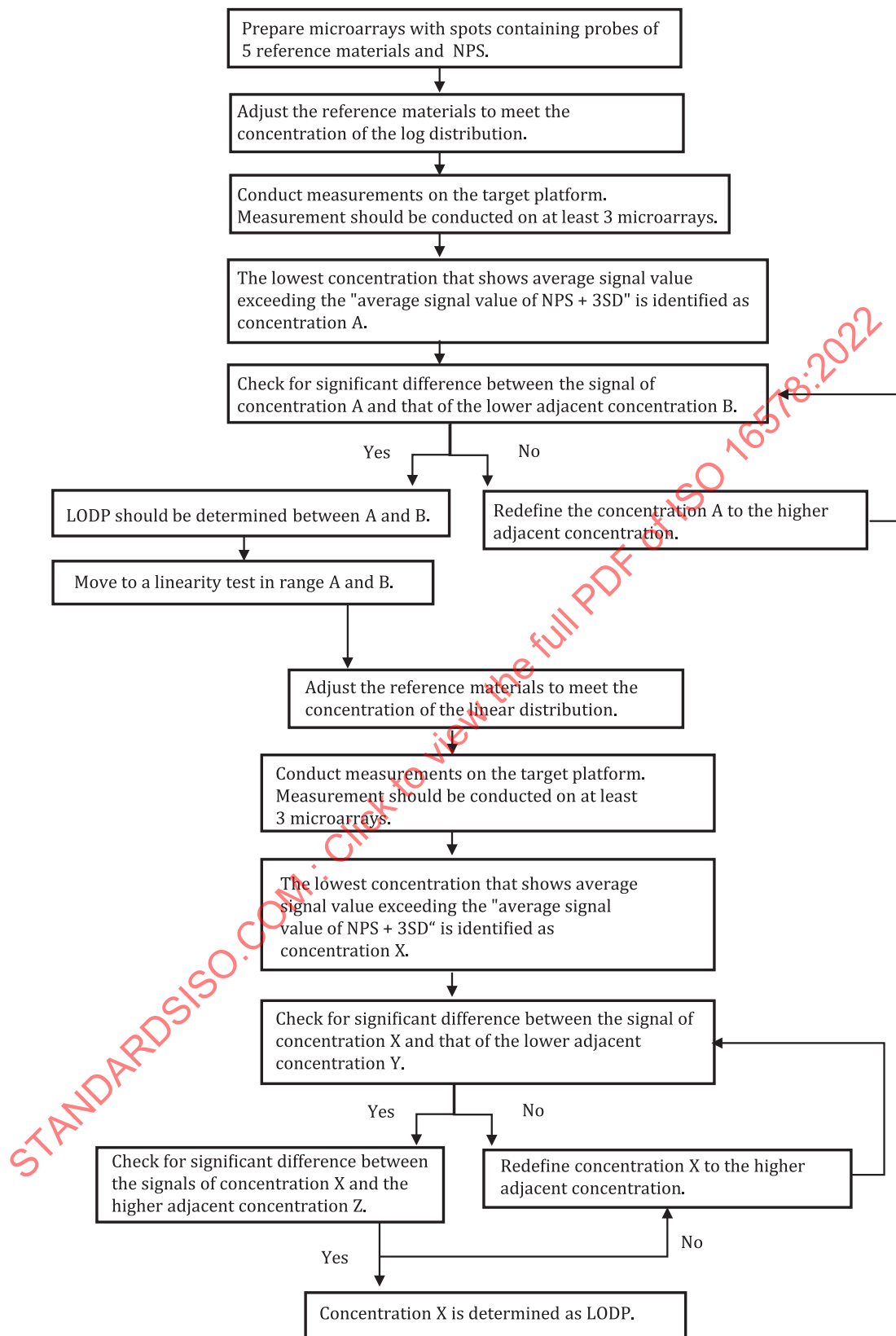
Figure A.1 — Flowchart for LODP determination
