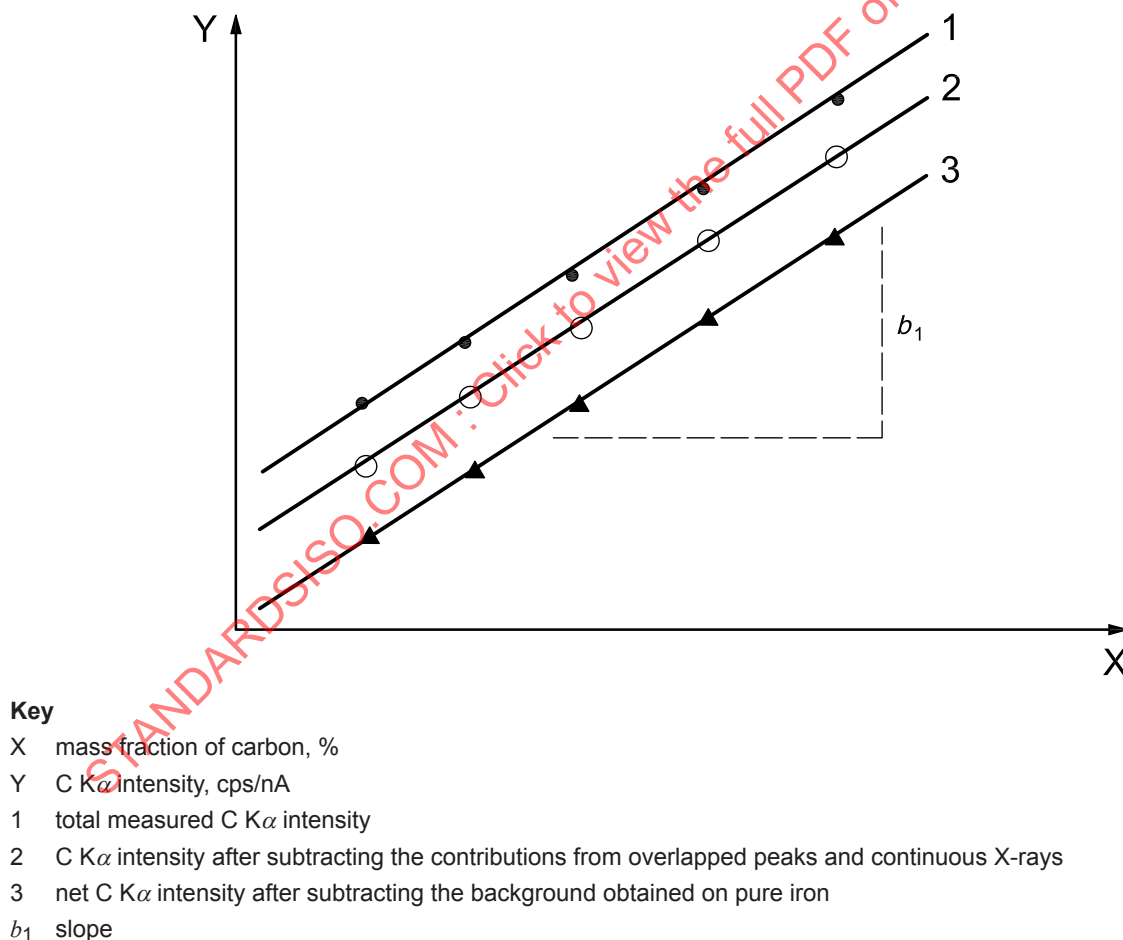
Figure 3 — Calibration curve for determining carbon content in steels
