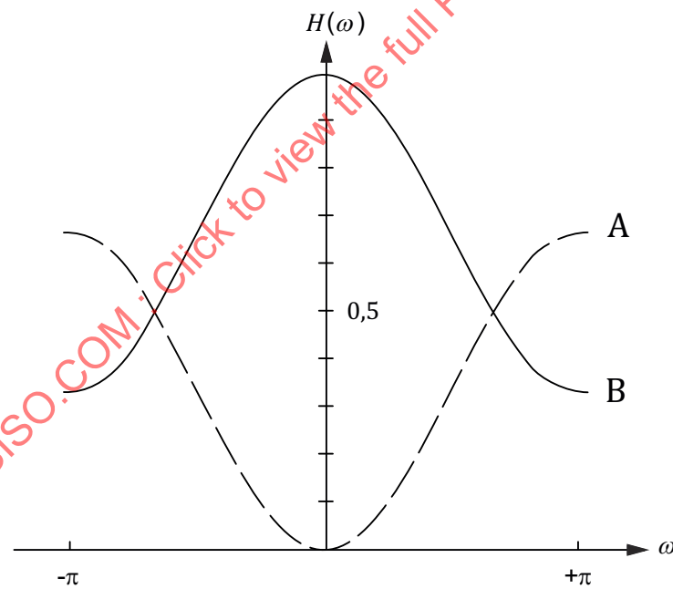
Figure 3 — Transfer function of the moving average filter of length 3
