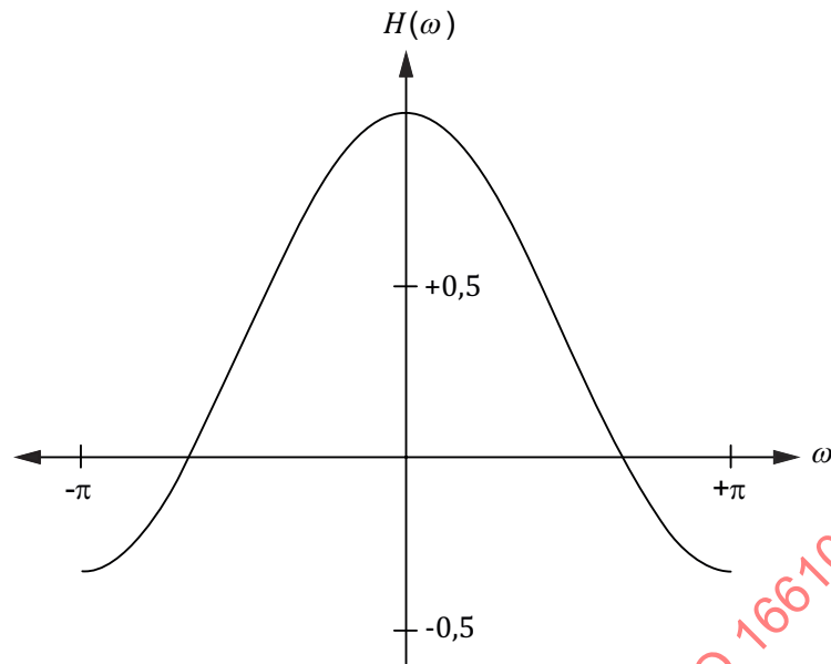
Figure 3 — Transfer function of the moving average filter of length 3
