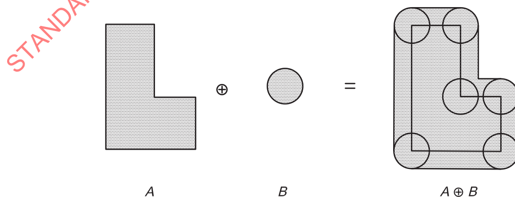
Figure 1 — Minkowski addition of two sets
