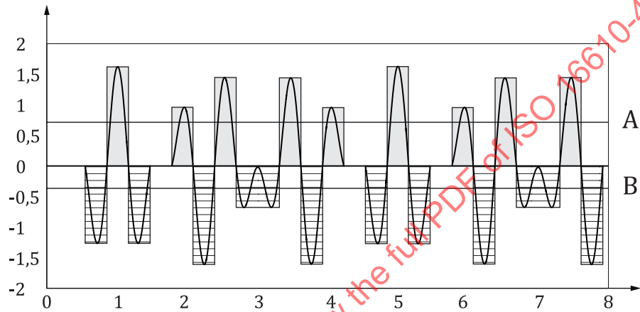
b) Set profile elements to zero which meet the discrimination criteria
