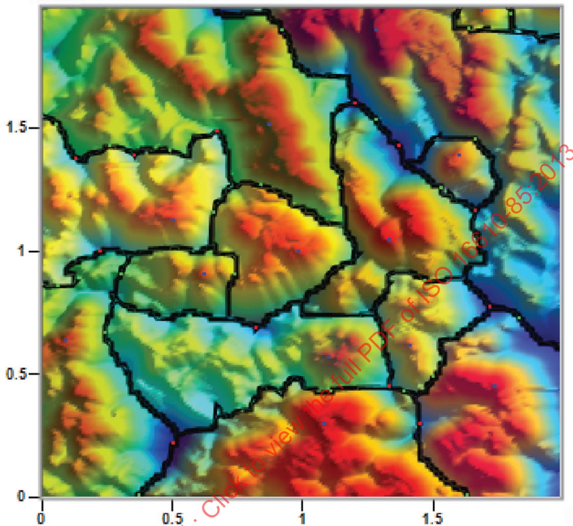
Figure 5 — Example of segmentation of a surface from a grinding wheel with Wolf pruning 15 % total height
