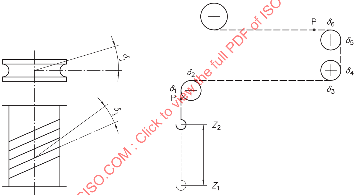
Figure 9 — Fleet angles
