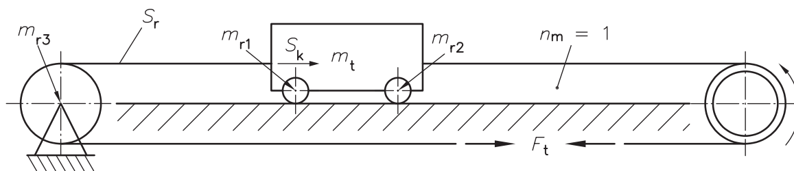
b) Example for general rope drive including rope pre-tension
