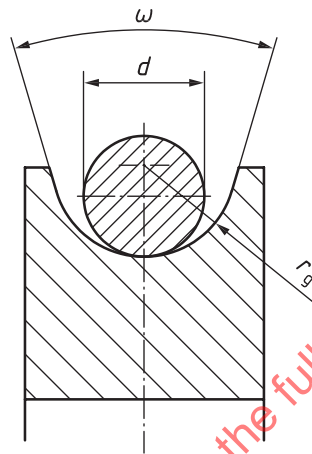
Figure 10 — Groove
