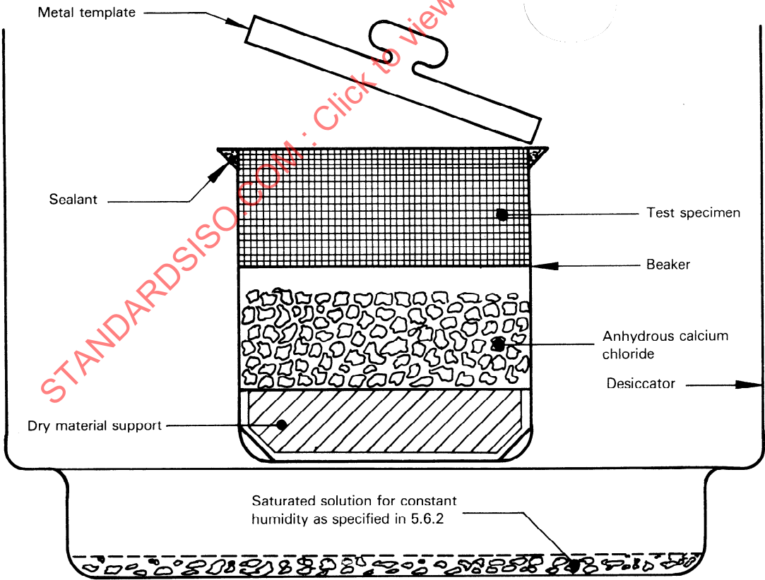
Figure — Example of mounted specimen in test beaker and constant-humidity desiccator
