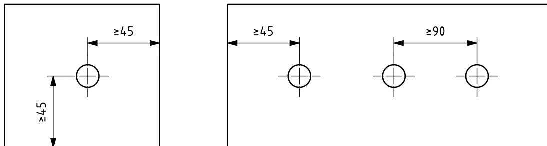
Figure 2 — Dimensions of the test pieces
