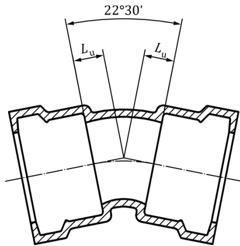
Figure 11 — Double socket bend 22°30' (1/16)
