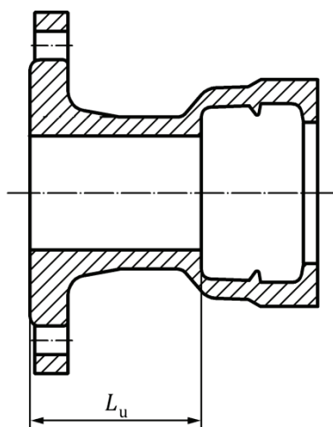
Figure 6 — Flanged socket
