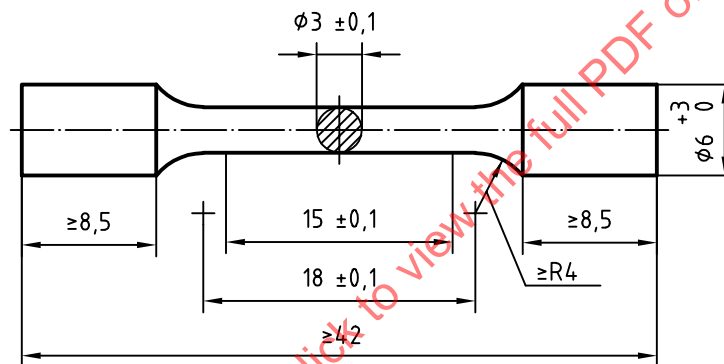
Figure 2 — Test specimen with radial shoulders
