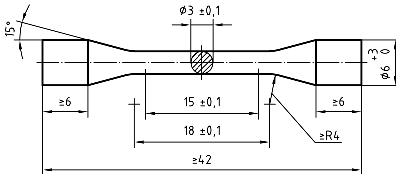
Figure 1 — Test specimen with conical shoulders
