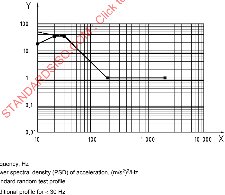
Figure 11 — PSD vs. frequency
