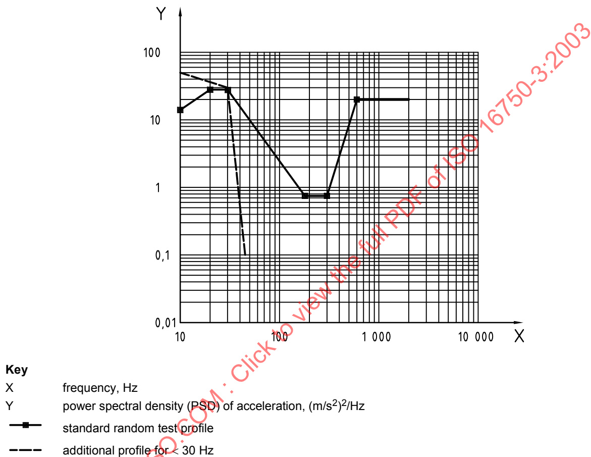
Figure 10 — PSD vs. frequency
