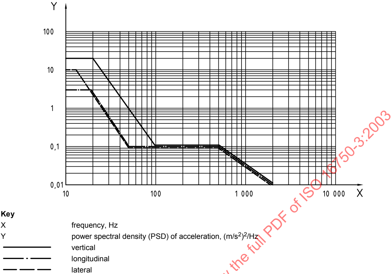
Figure 12 — PSD vs. frequency
