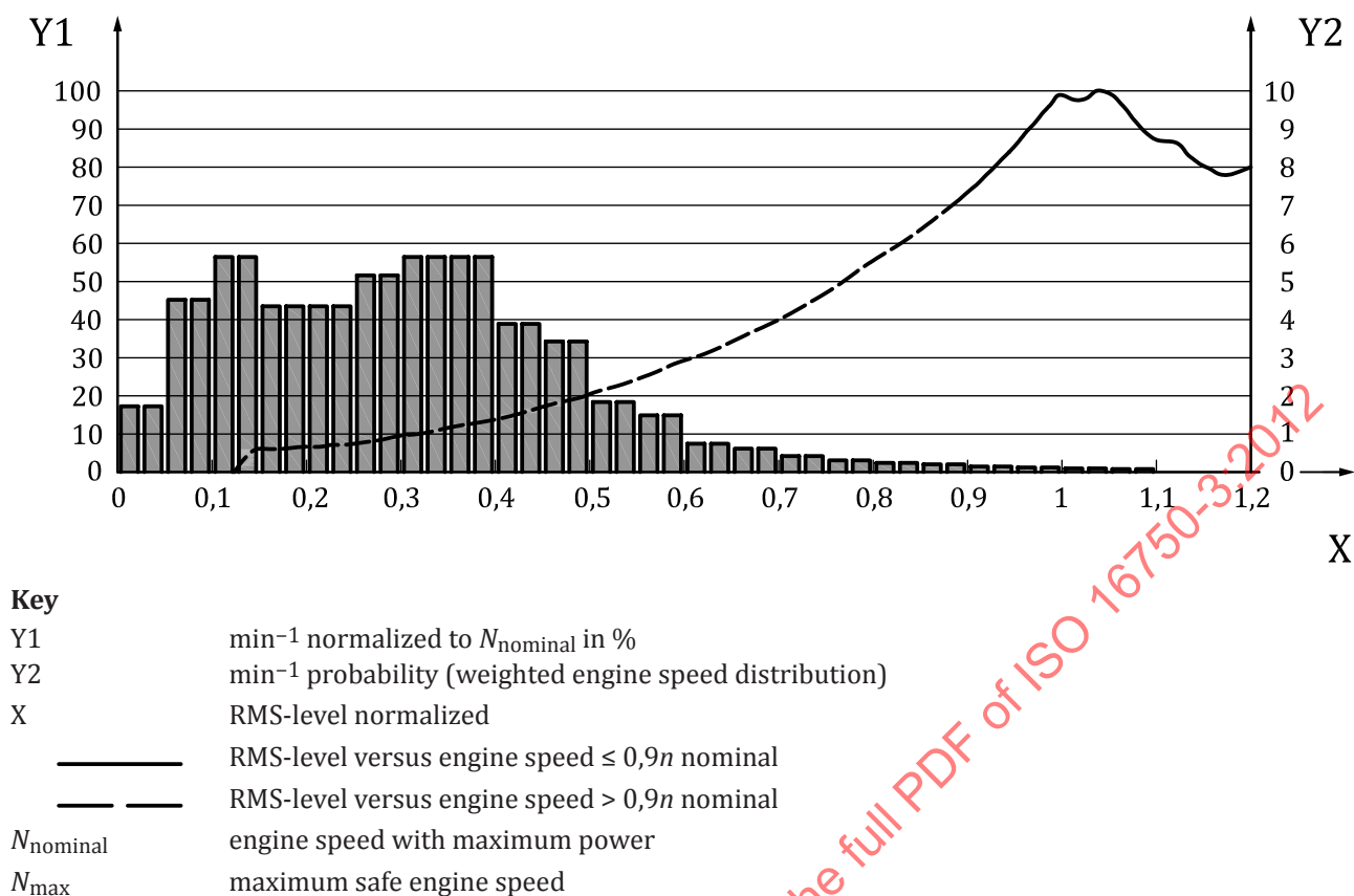
Figure A.1 — RMS-acceleration level and weighted min -1 distribution versus engine speed
