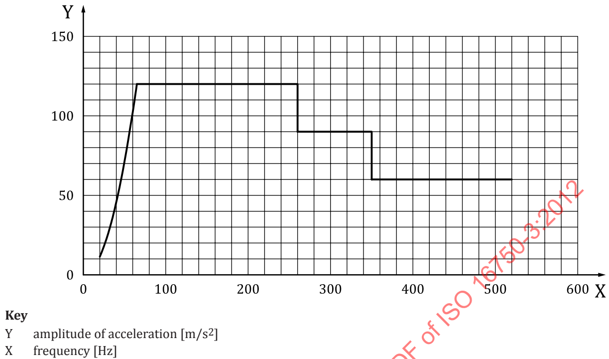
Figure 9 — Max. acceleration versus frequency
