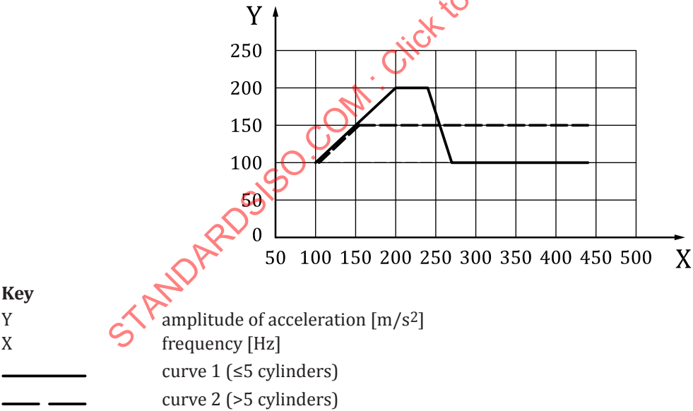
Figure 2 — Vibration severity curves
