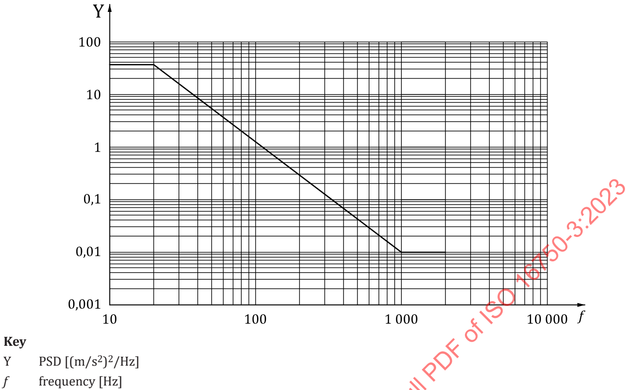
Figure 18 — PSD of acceleration versus frequency
