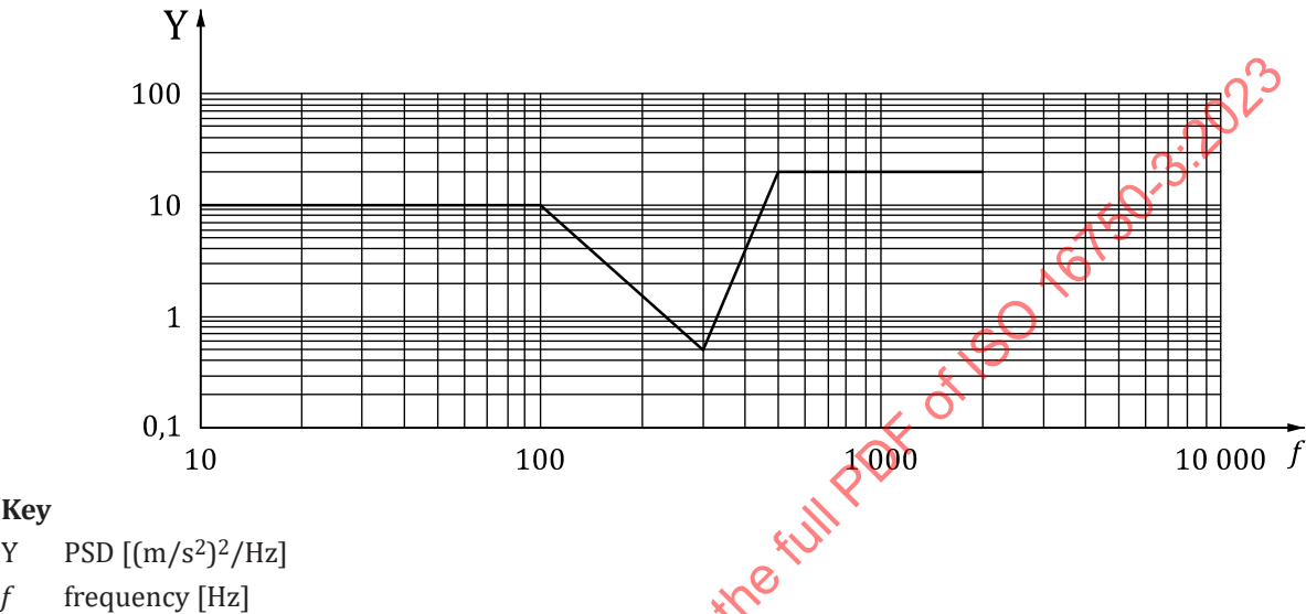
Figure 5 — PSD of acceleration versus frequency
