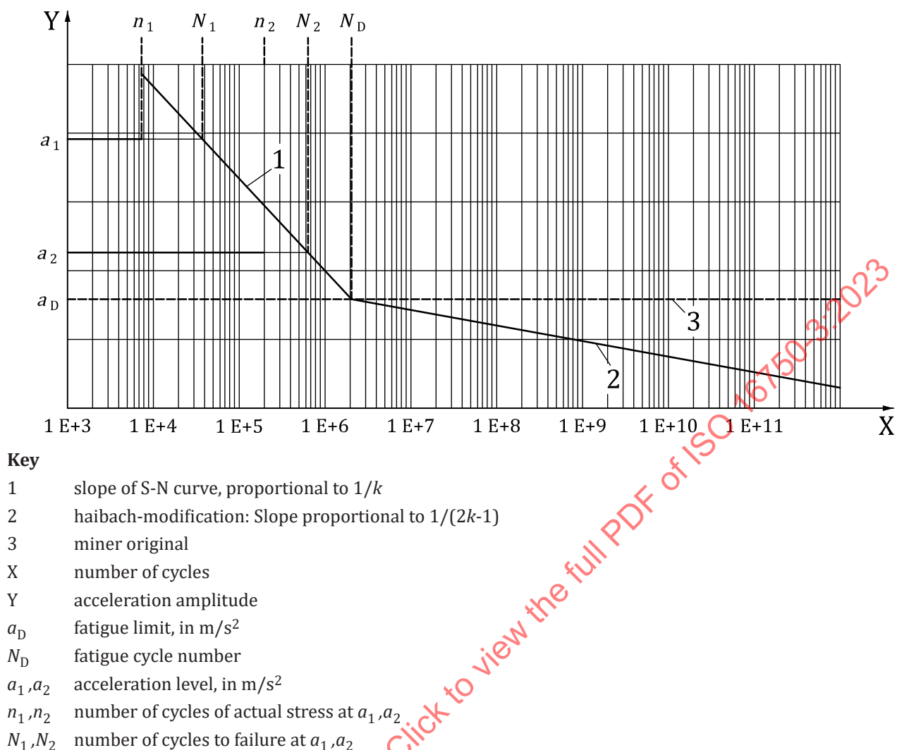
Figure A.8 — Haibach hypotheses — Linear damage accumulation “S”
