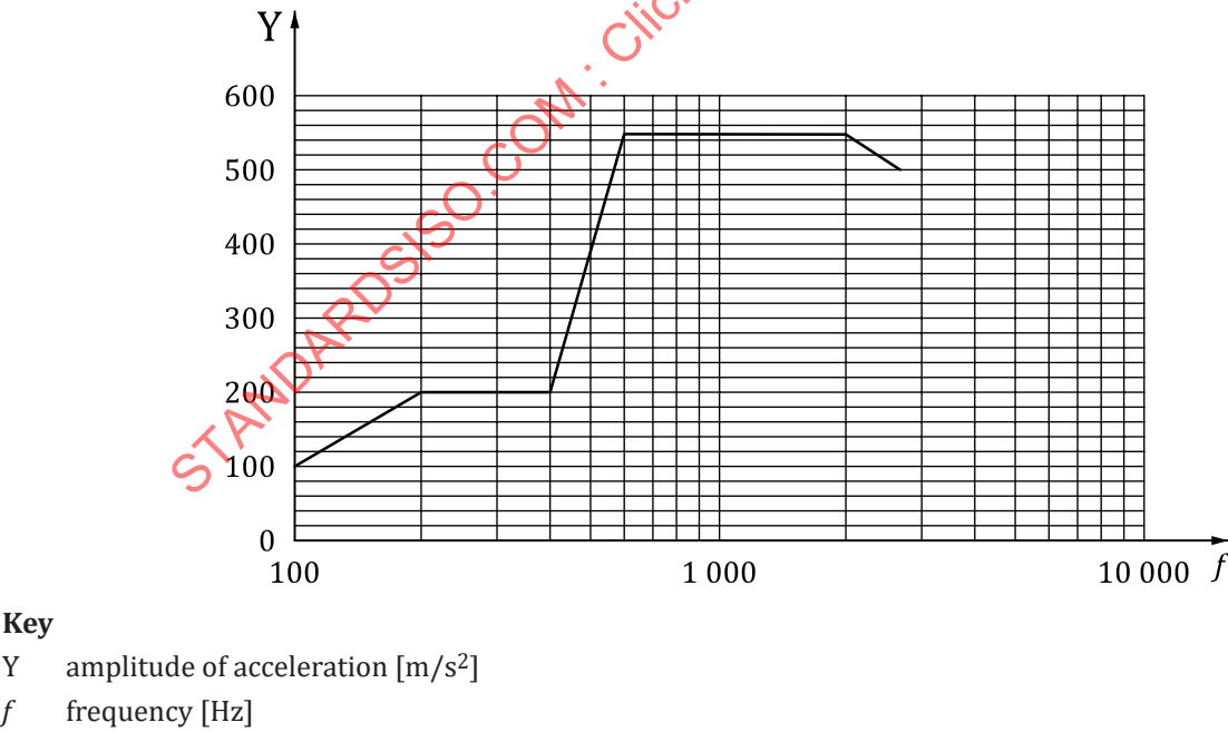
Figure 29 — Acceleration versus frequency
