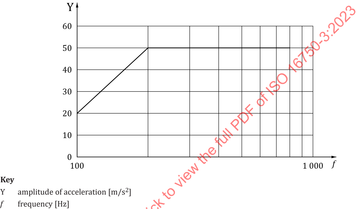
Figure 24 — Acceleration versus frequency
