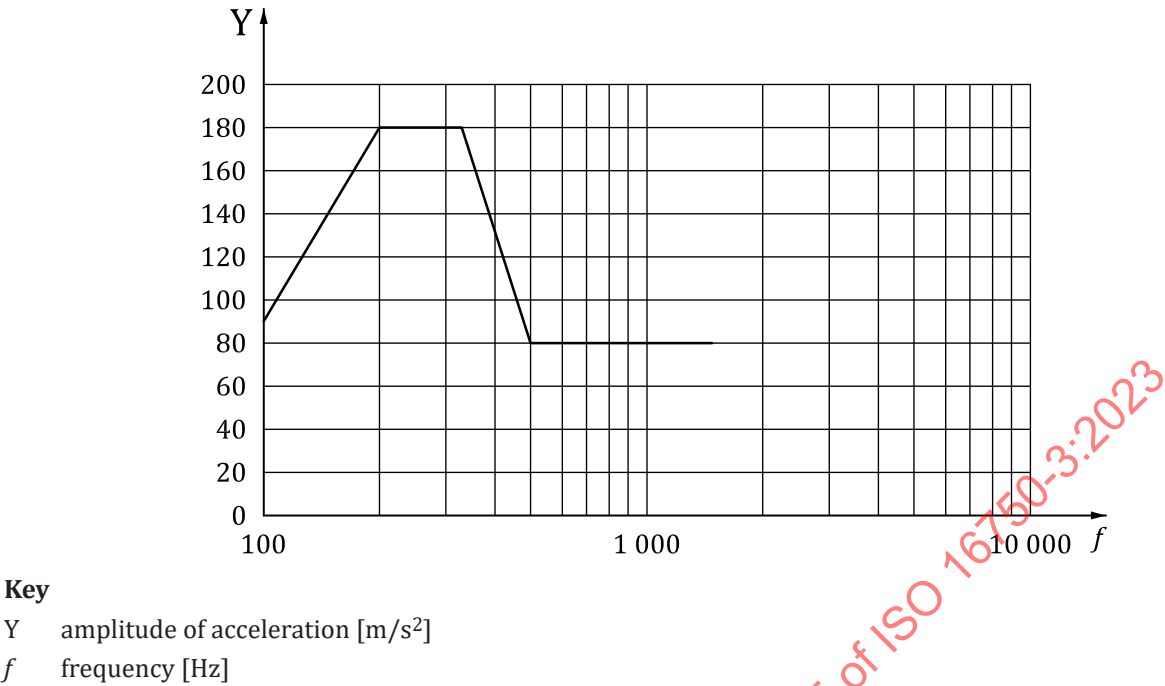
Figure 21 — Acceleration versus frequency
