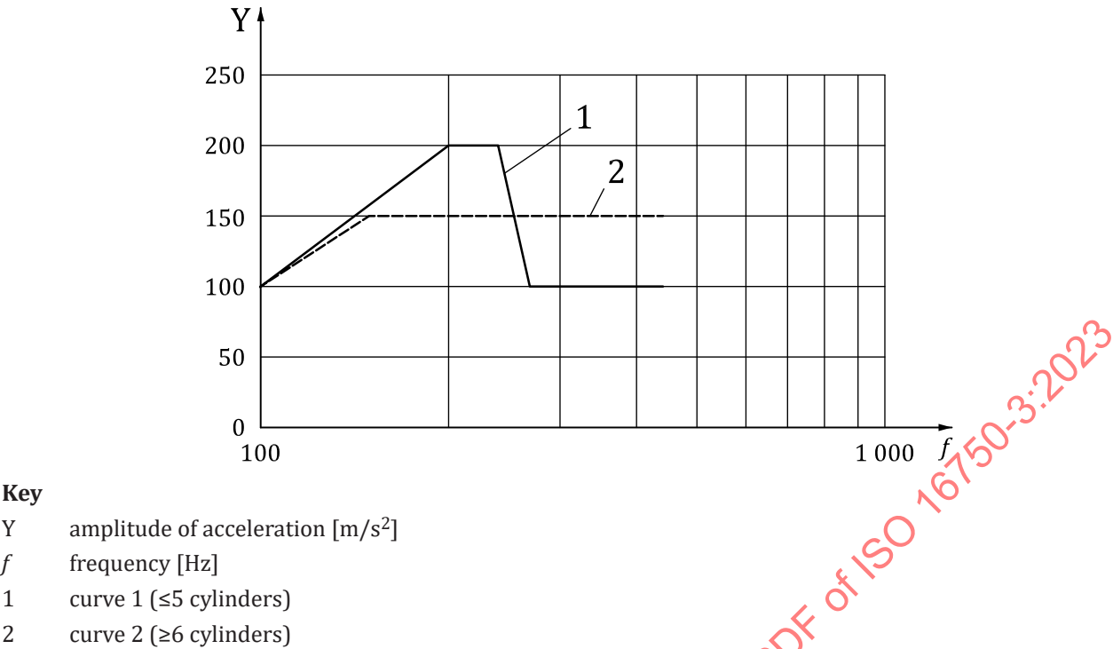
Figure 4 — Acceleration versus frequency
