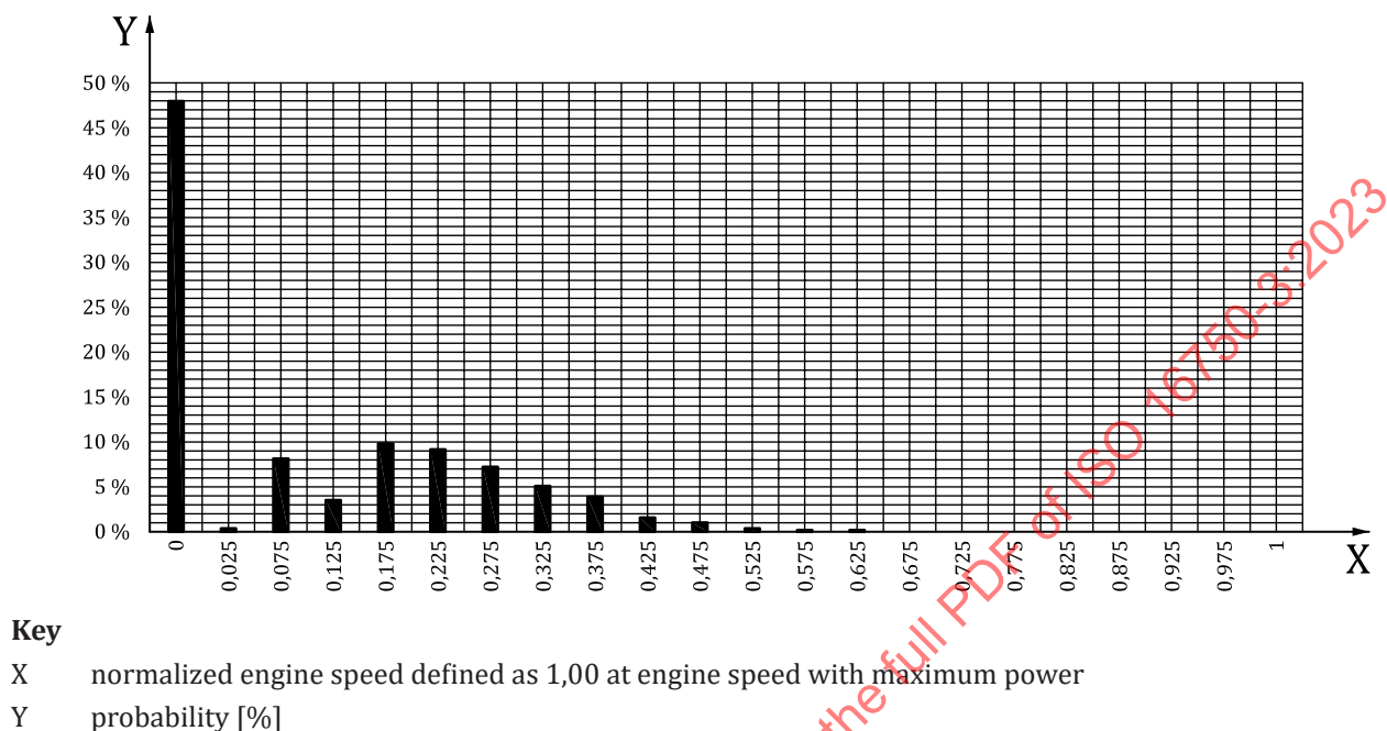
Figure A.4 — Engine speed distribution in a PHEV
