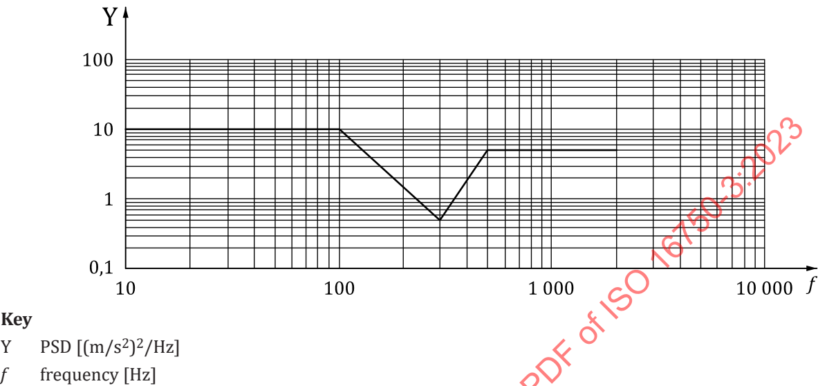
Figure 7 — PSD of acceleration versus frequency
