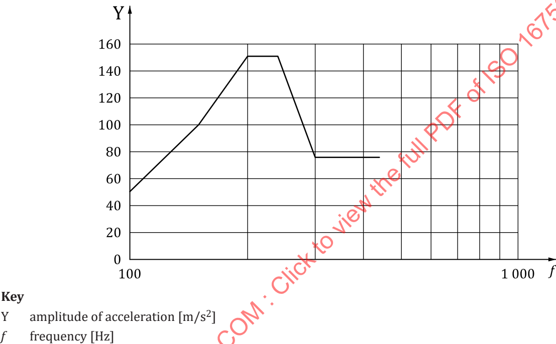
Figure 22 — Acceleration versus frequency
