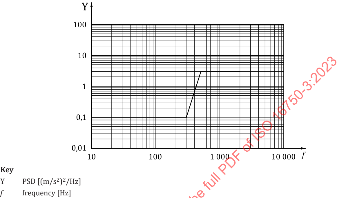
Figure 11 — PSD of acceleration versus frequency
