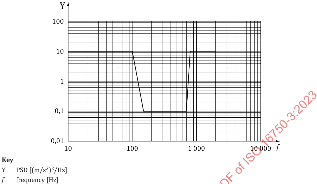
Figure 25 — PSD of acceleration versus frequency
