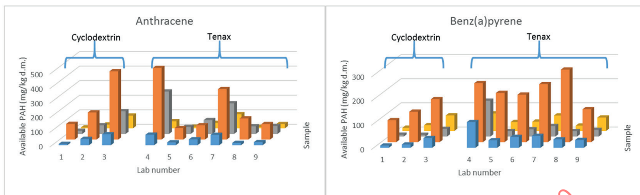
Figure C.1 — Bioavailability of Anthracene and Benz(a)pyrene. Results of cyclodextrin and Tenax extraction of participating laboratories in four samples
