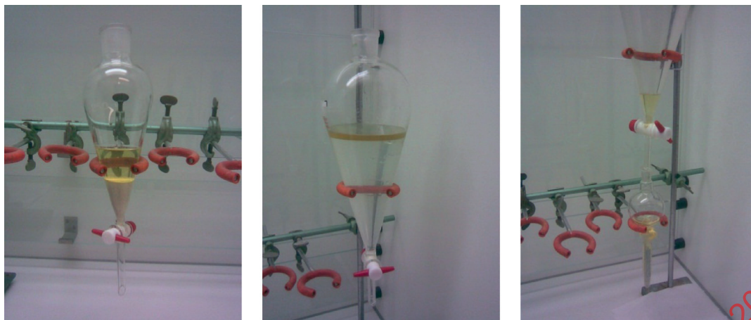
Figure B.3 — Extraction of the Tenax ® and collection of the petroleum ether phase (see 7.4.4)
