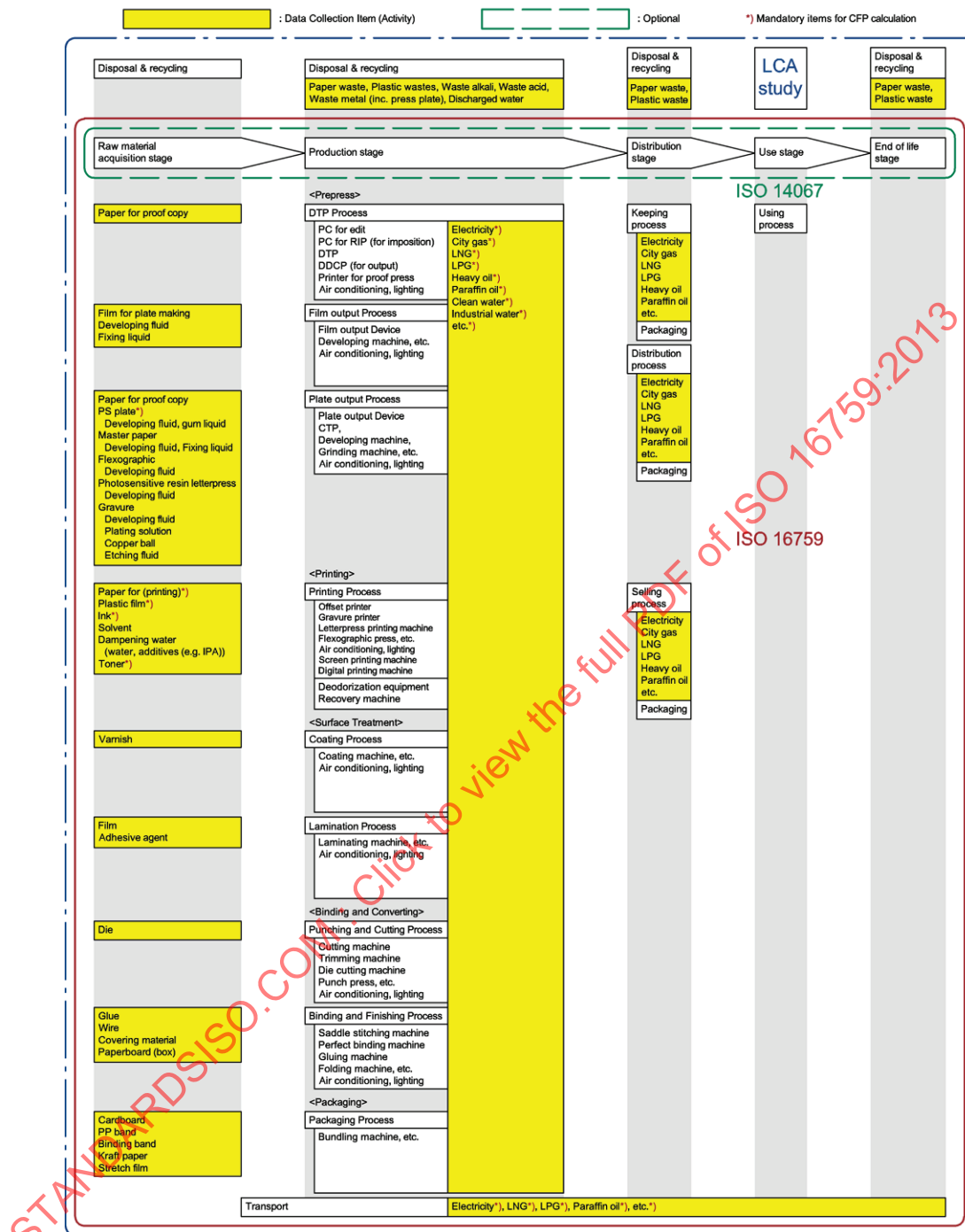
Figure C.1 — Data collection and system boundary for carbon footprint of print media products
