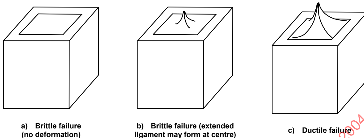
Figure 1 — Failure surfaces
