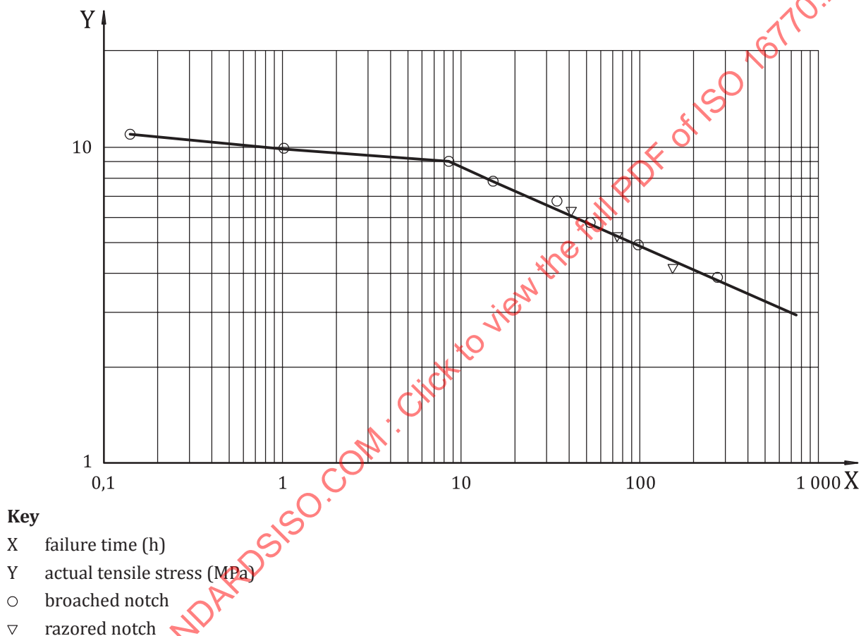
Figure 6 — Typical stress/failure time plot
