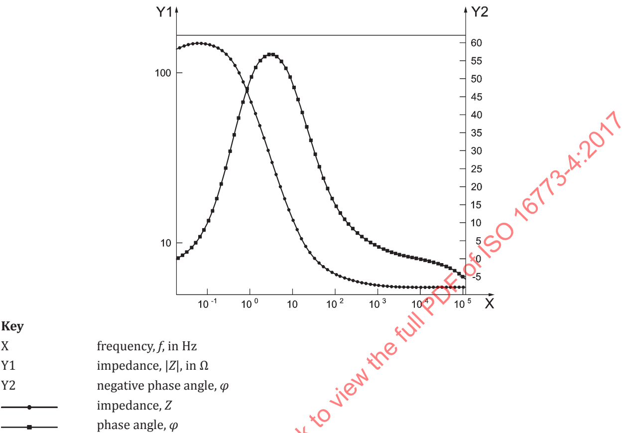
Figure A.17 — Bode plot for alkaline degreased cold rolled steel
