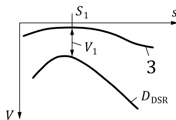
b) Gain difference for S_1
