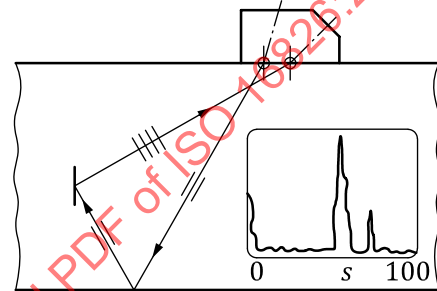
d) LLT probe on test object with typical evaluation
