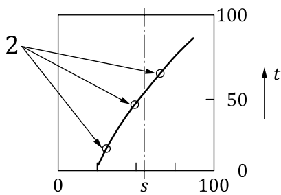
c) Diagram showing depth versus sound path
