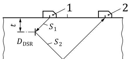
e) Combined sound path
