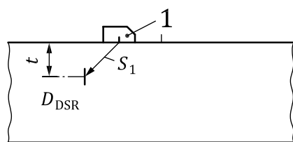
a) Sound path S_1
