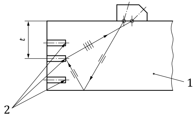
b) LLT probe on reference block with disc-shaped reflectors
