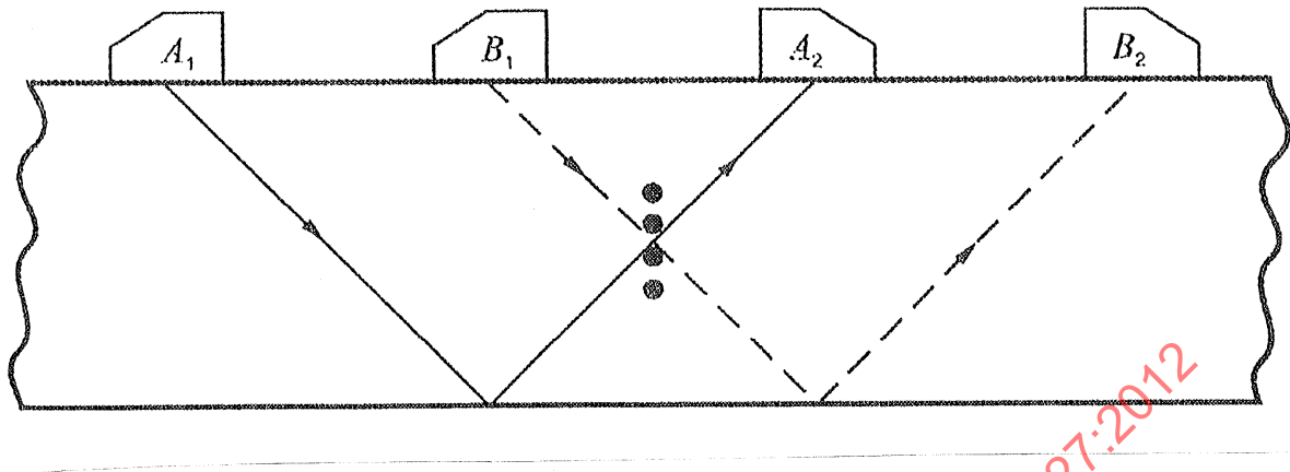
Figure 4 — Location of discontinuities by transmission technique using angle probes
