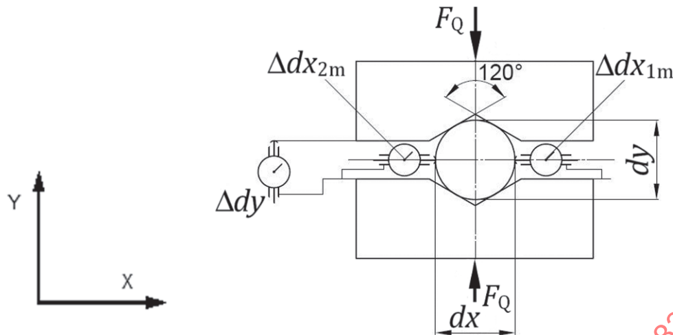
Figure 3 — Test set-up
