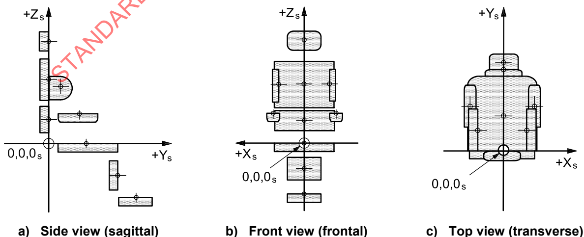
Figure 11 — Support surface axis system
