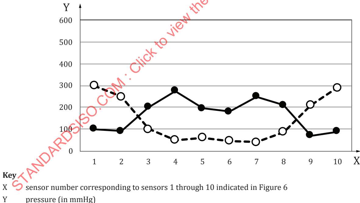
Figure 9 — Example of comparative line graph of pressure readings from the centre line of sensors for two different cushions
