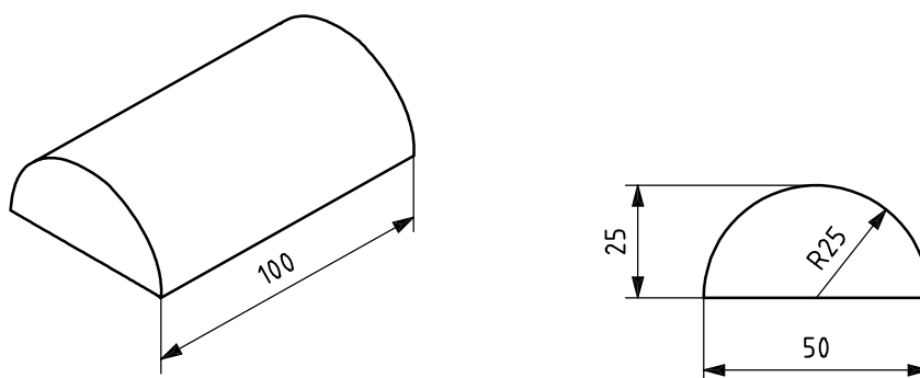
Figure 9 — Example of a convex loading pad
