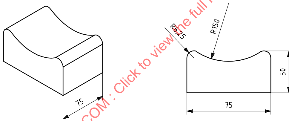
Figure 10 — Example of concave loading pad
