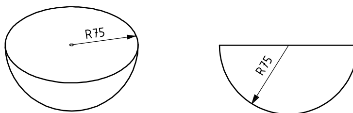
Figure 11 — Example of convex hemispherical loading pad
