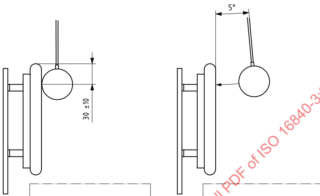
Figure 20 — Back support impact test alignment and set-up
