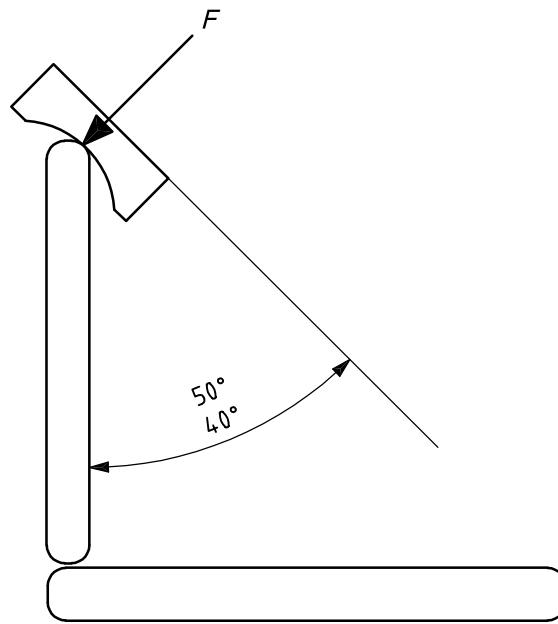
Figure 18 — Example of posterior force application to back support
