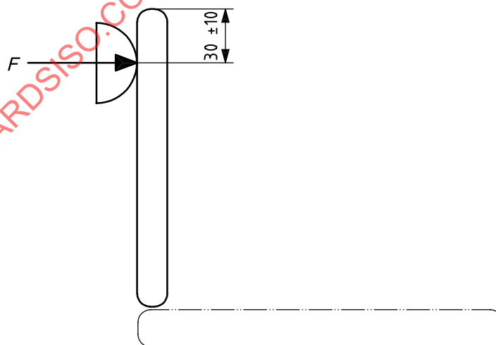
Figure 19 — Example of anterior force application to back support
