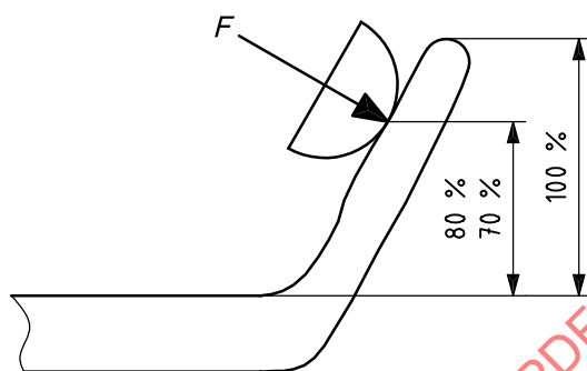
Figure 12 — Example of force application to lateral support continuous with the adjacent support surface
