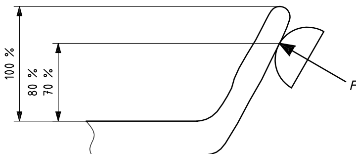
Figure 14 — Example of force application to lateral support continuous with the adjacent support surface
