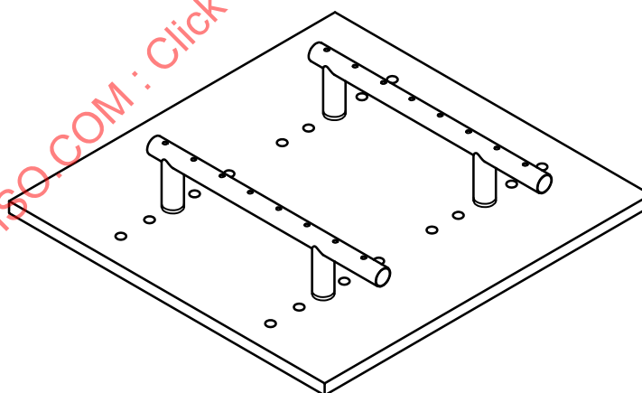
Figure D.1 — Example of adjustable rigid test frame, with mounting bars attached parallel to a base
