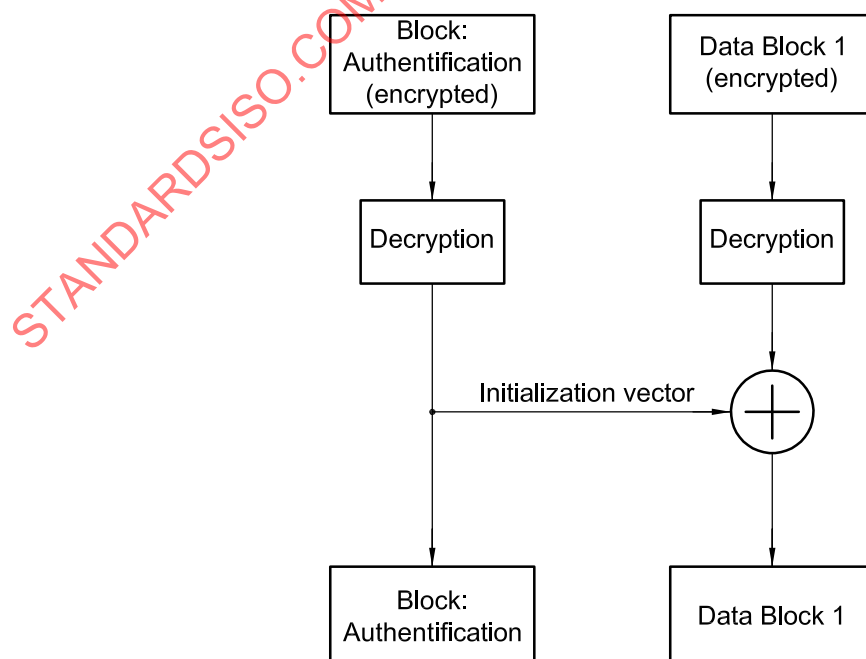
Figure 34 — Data block chaining — Decryption with two data blocks
