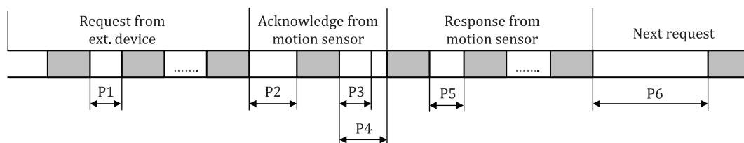
Figure 8 — Structure of timing during normal operation
