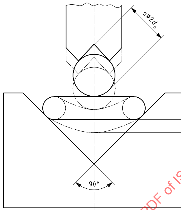
Figure 2 — Bend deflection, f
