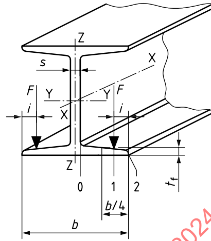
b) I-beam with tapered flanges
