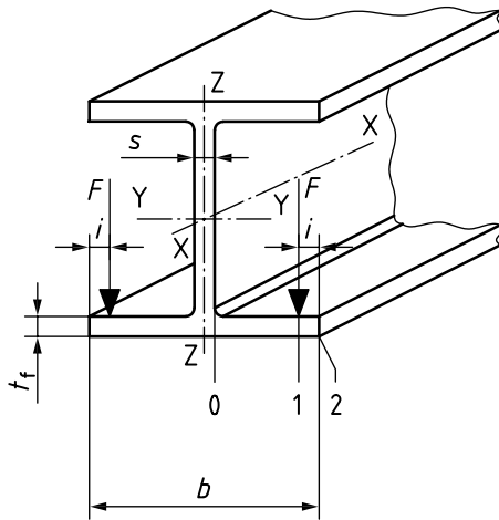
a) I-beam with flanges of uniform thickness
