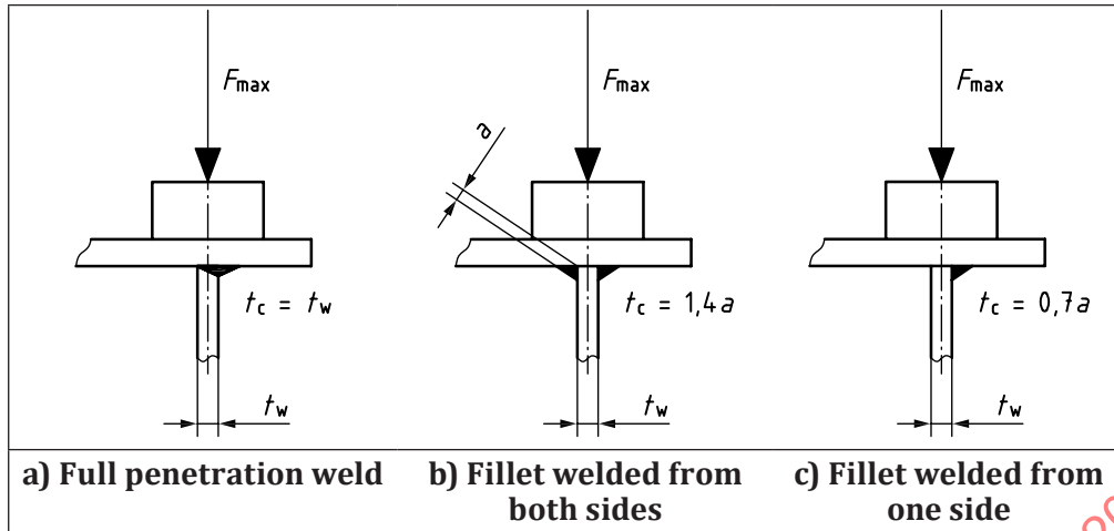
Figure A.1 — Description of t_w and t_c
