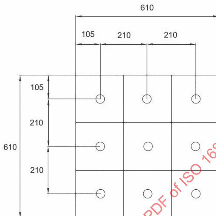
Figure 9 — Air velocity and aerosol uniformity sampling points
