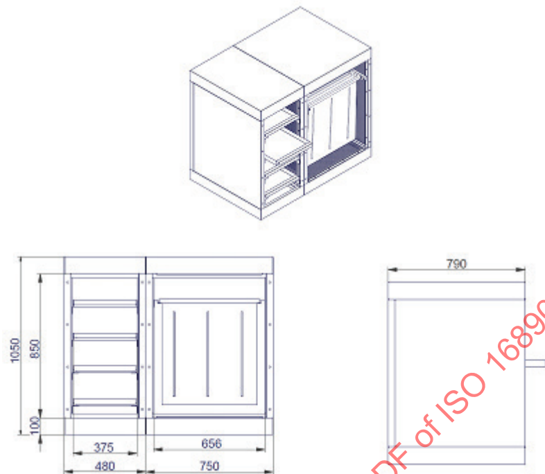
Figure 1 — Conditioning cabinet schematic drawing
