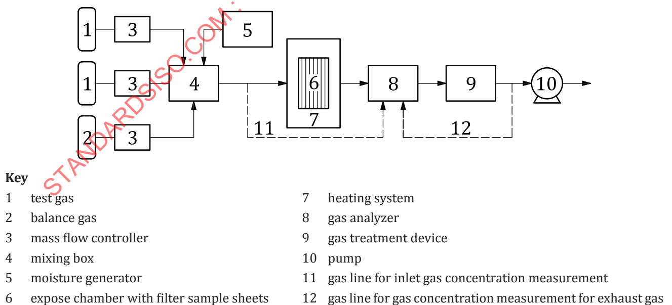
Figure 5 — Example of continuous flow through type setup for exposure test
